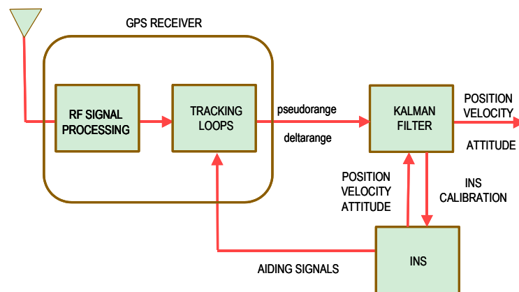
Figure 16. Tightly coupled approach.
