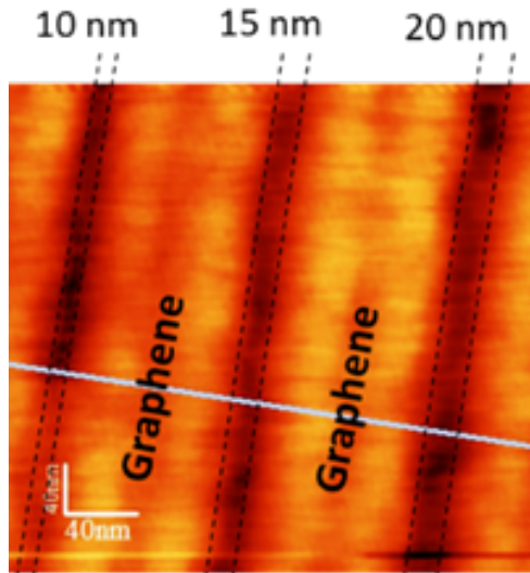
Figure 57: Atomic Force Micrograph of the 10, 15 and 20 nm graphene slits developed using the optimized method after PMMA removal in forming gas annealing.
