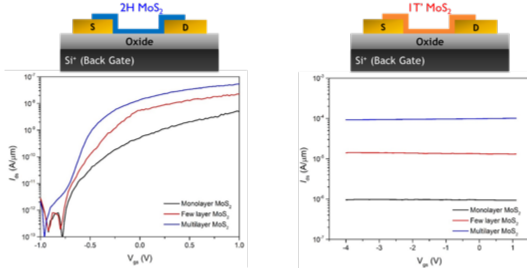
Figure 69: Transfer characteristics of backgated MoS 2 FETs for different channel thickness before and after phase transition.
