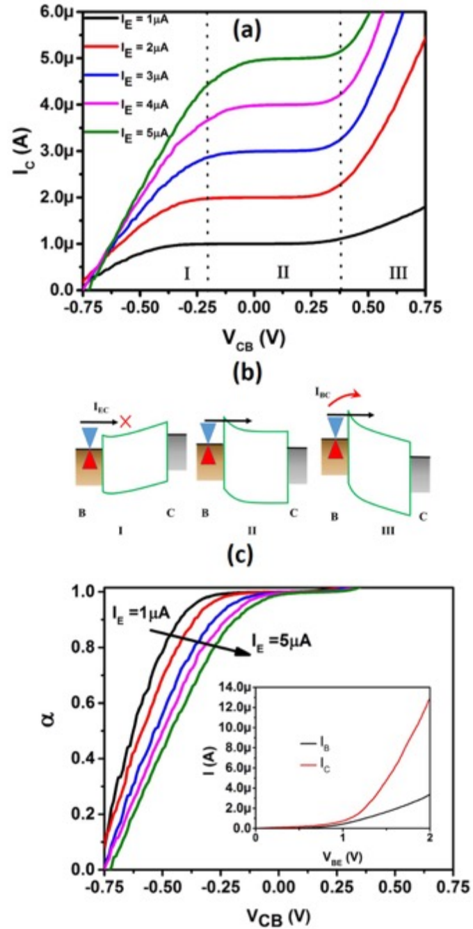
Figure 39(a) Common-base characteristics of the device A and (b) corresponding schematic energy band diagrams in different operating regions(c) Injection ratio for device A for different emitter injection currents. Inset shows the Gummel plot for V_{cb} = 0 V.
