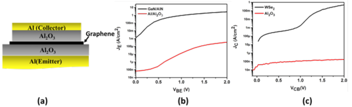
Figure 38. (a) Schematic cross-section of the fabricated HET with \text{Al}_2\text{O}_3 as dielectric barriers (b) J-V comparison of GaN/AlN/graphene and Al/ \text{Al}_2\text{O}_3 /graphene diodes. (c) Characteristics comparison showing J_c vs V_{cb} between a \text{WSe}_2 -based and an \text{Al}_2\text{O}_3 -based B-C diode.
