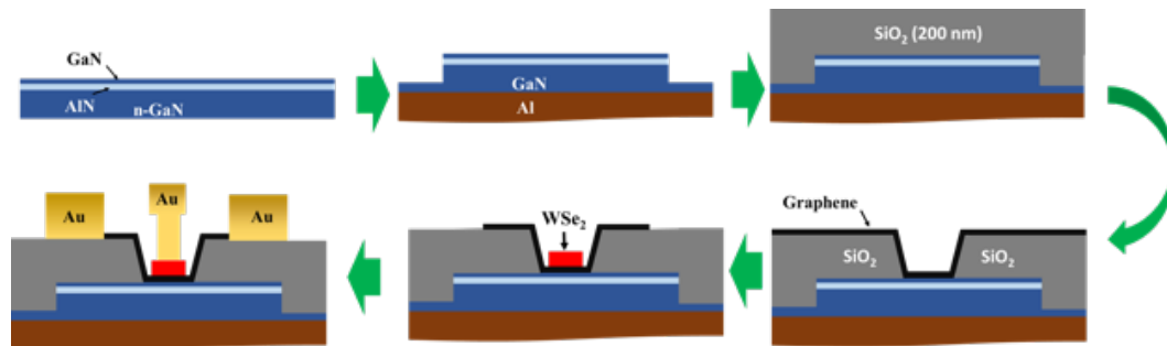
Figure 36 Schematic illustration of HET fabrication process.
