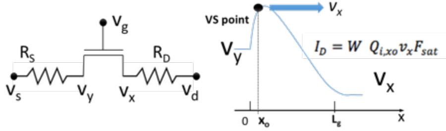
Figure 84. The concept of virtual source injection modeling
