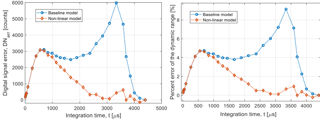
Figure 33. Signal error of the Sensor response to incident light for the baseline and non-linear model at several integration times spanning the full dynamic range for (right) the digital signal percent error of the dynamic range and (left) the signal error in counts.
