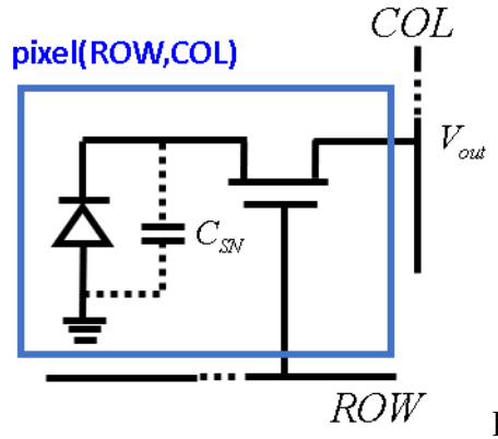
Figure 10. Schematic of a CMOS Passive Pixel Sensor (PPS).
