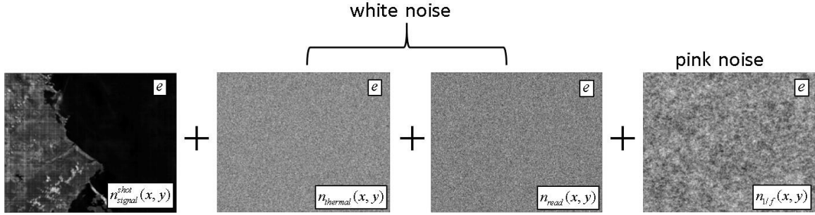
Figure 5. Example on how the total signal is obtained in ASSET. Noise components are added to the detector frame n_{signal}^{shot} to obtain the total analog signal in electrons. From left to right: Total signal after shot noise, thermal noise, read noise, and flicker noise. Also shown are the units and the distribution used for each noise.
