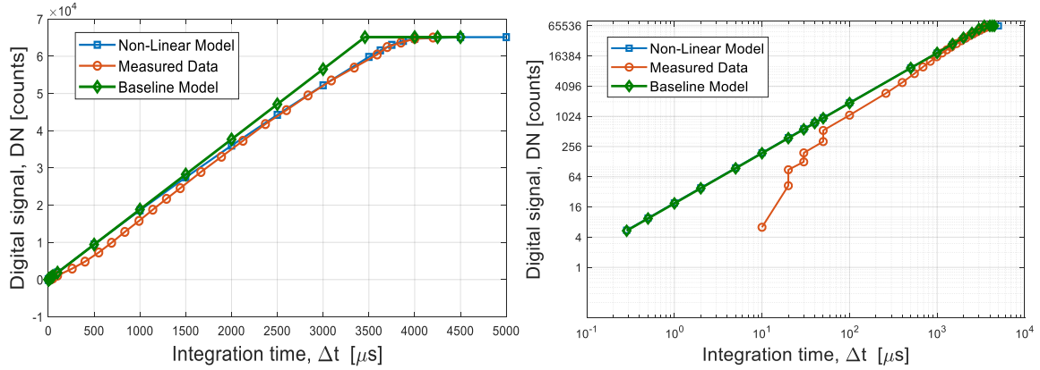
Figure 32. Sensor response to incident light for measured, baseline and non-linear models at several integration times spanning the full dynamic range for (left) linear and (right) logarithmic scales.
