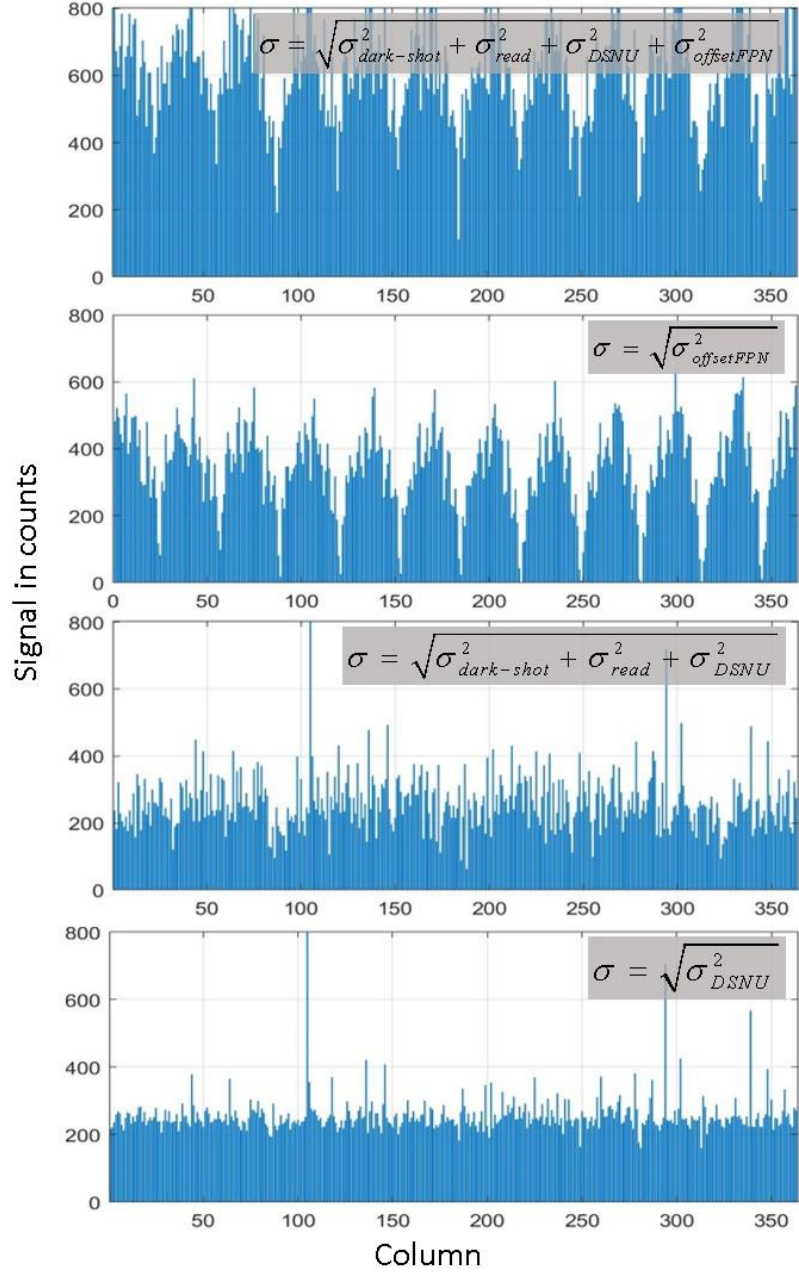
Figure 42. Phantom v12.1 array signal values (DN) for all columns of one row. From top to bottom: single dark frame at 30 ms integration time, average of 500 bias frames at 0.285 \mu\text{s} , difference between single dark frame and average bias frame, and average of 500 dark frames at 30 ms after offset FPN subtraction. Also shown are the associated RMS noise ( \sigma ) and its components. One can note from the figure that there are 32 columns periodic FPN present in the near-zero integration time offset (presumably due to differences in ADCs) whereas DSNU is relatively uniform across the column.
