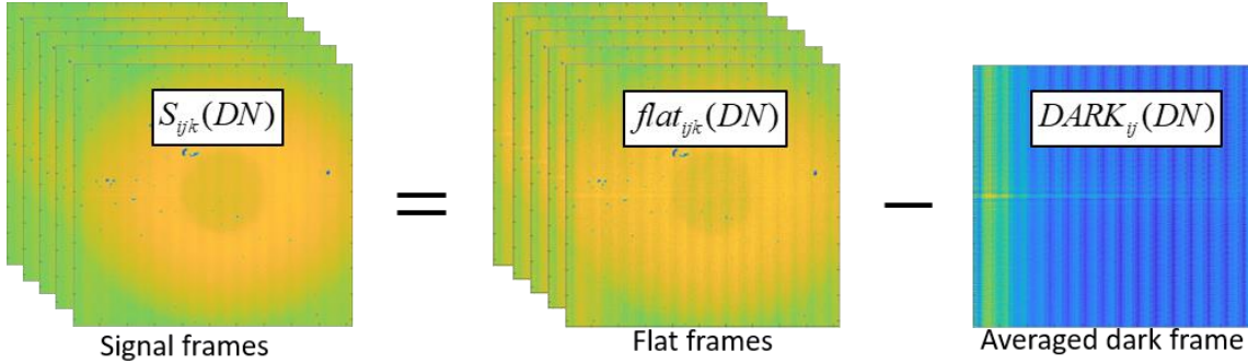
Figure 26. Illustration showing how the signal frames are obtained by subtracting an averaged dark frame from the flat frames.
