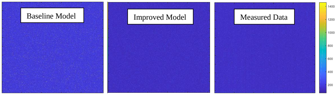
Figure 44. Comparison of an averaged dark signal frame for the baseline model with a normal distribution (left), the improved model with a log-normal distribution (center), and the measured (right) data for integration time \Delta t = 30 ms.
