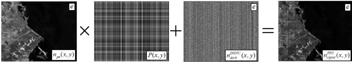
Figure 3. Examples of non-uniformities in ASSET; PRNU is multiplied by the photogenerated signal and electrons due to dark signal are added to obtain the detector frame with FPN. To account for perturbations due to the non-uniformities in the detector, the detector frame is multiplied by the PRNU and electrons due to dark signal are added.
