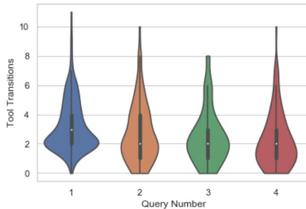
Figure 4.18: Tool Transitions versus Query Number
