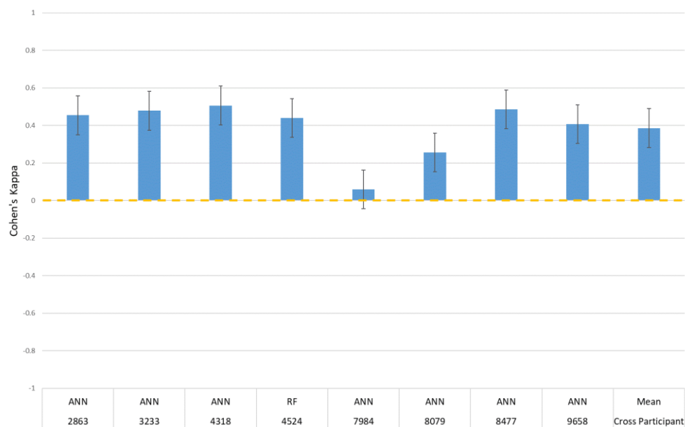
Figure 4.5: Cohen's Kappa for the Best Performing Models on the RDK Task
