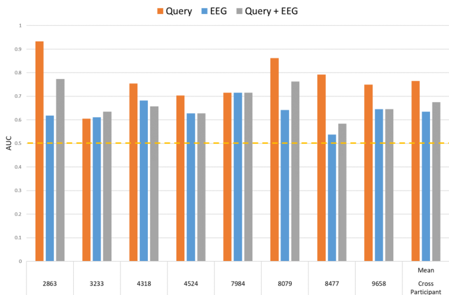
Figure 4.29: Comparison of AUC When Controlling for Query
