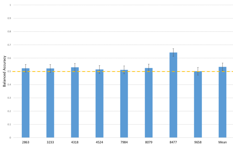
Figure 4.7: BACC for the CRNN fit on the RDK Task Data
