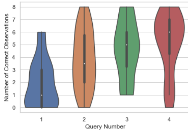
Figure 4.21: Number of Correct Observations versus Query Number
