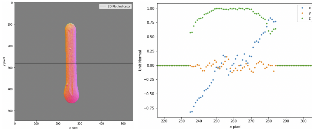
Figure 23. A normal map representing a sample's surface orientation (left) and a 2D visual of the normals across the width of the sample (right).
