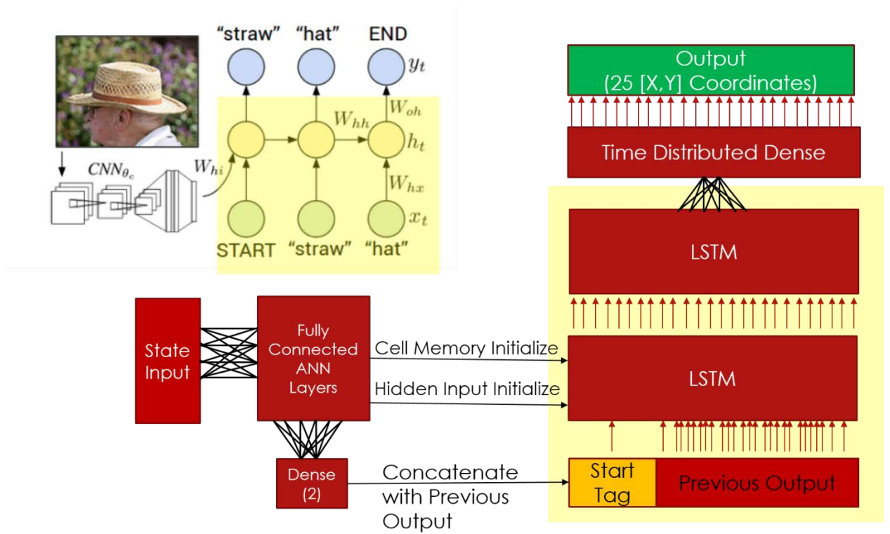
Image 14: Inspirational architecture analogous functionality – LSTM layers
