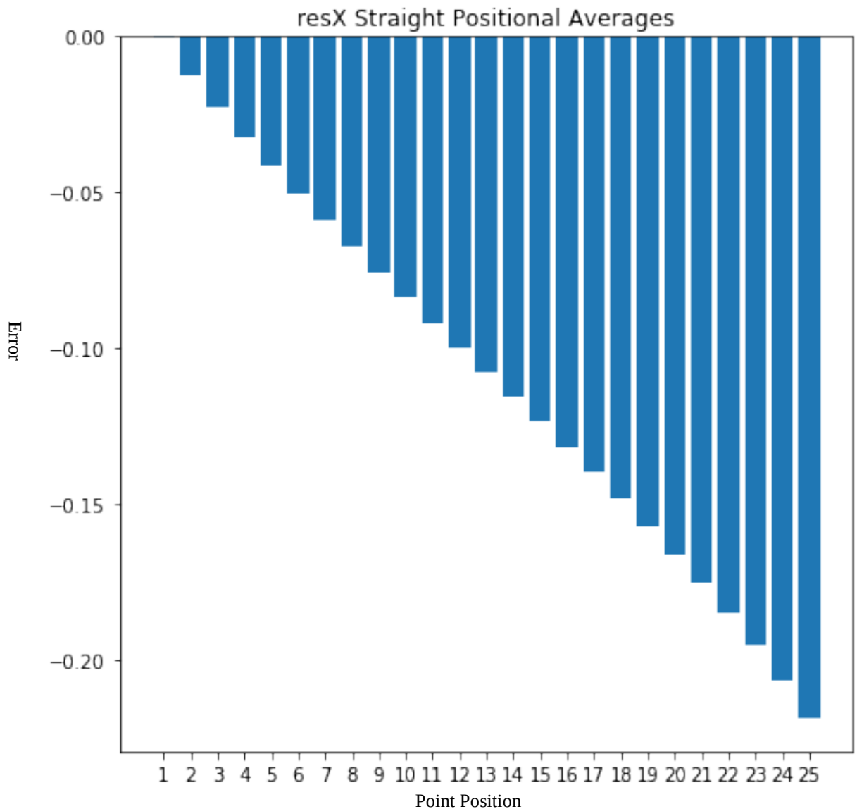
Figure 3: Data trajectory X value residual error averages
