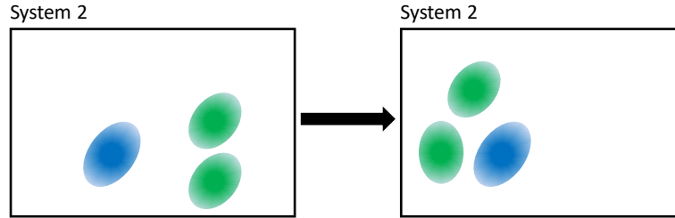
Figure 13: Concept drift.
