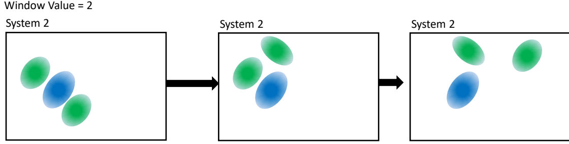
Figure 9: Windowing.
