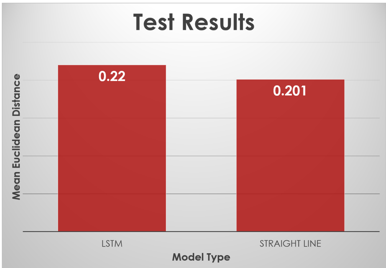
Figure 8: Test results
