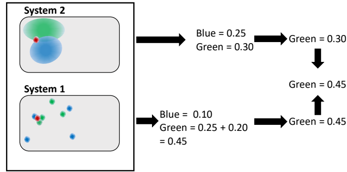
Figure 16: Inference.
