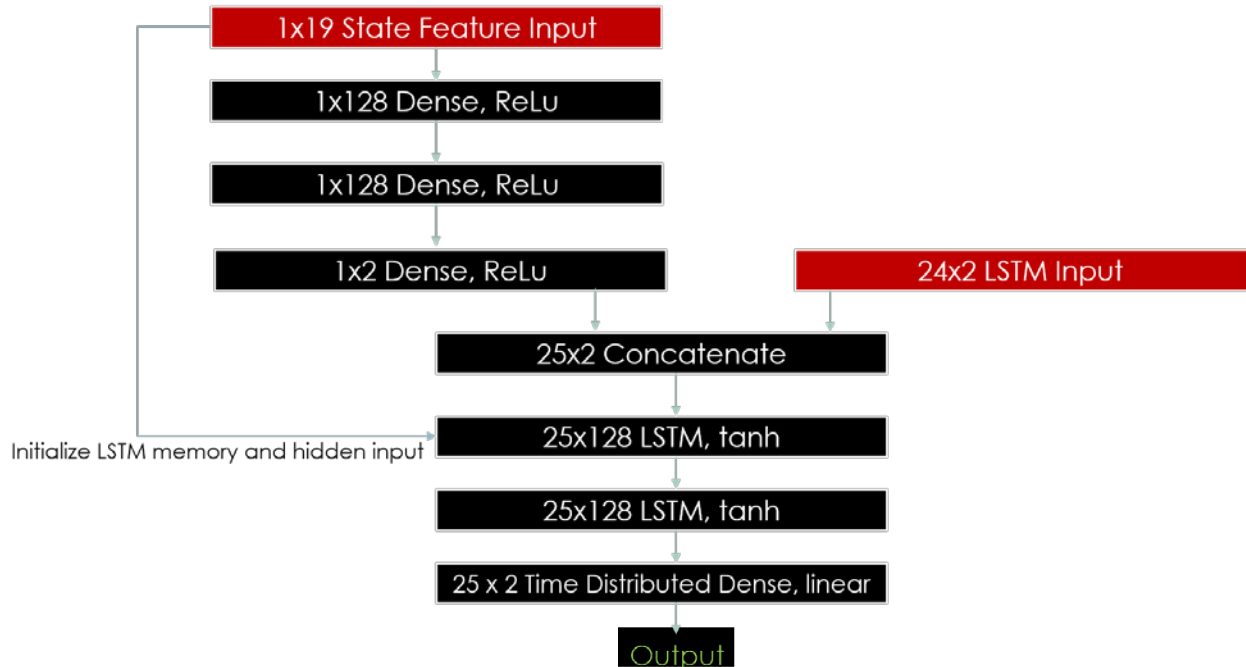
Image 11: Deep learning LSTM architecture – graph form
