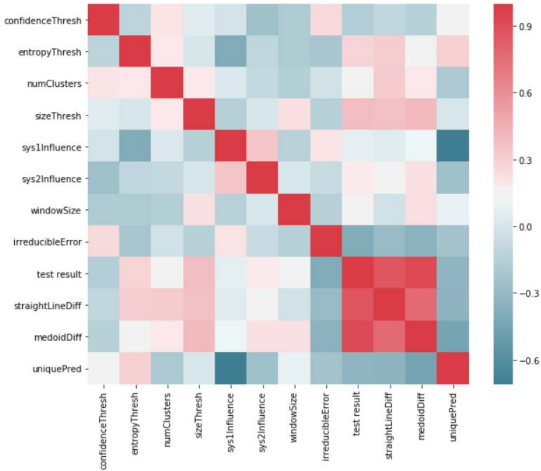
Figure 39: Correlation heatmap.
