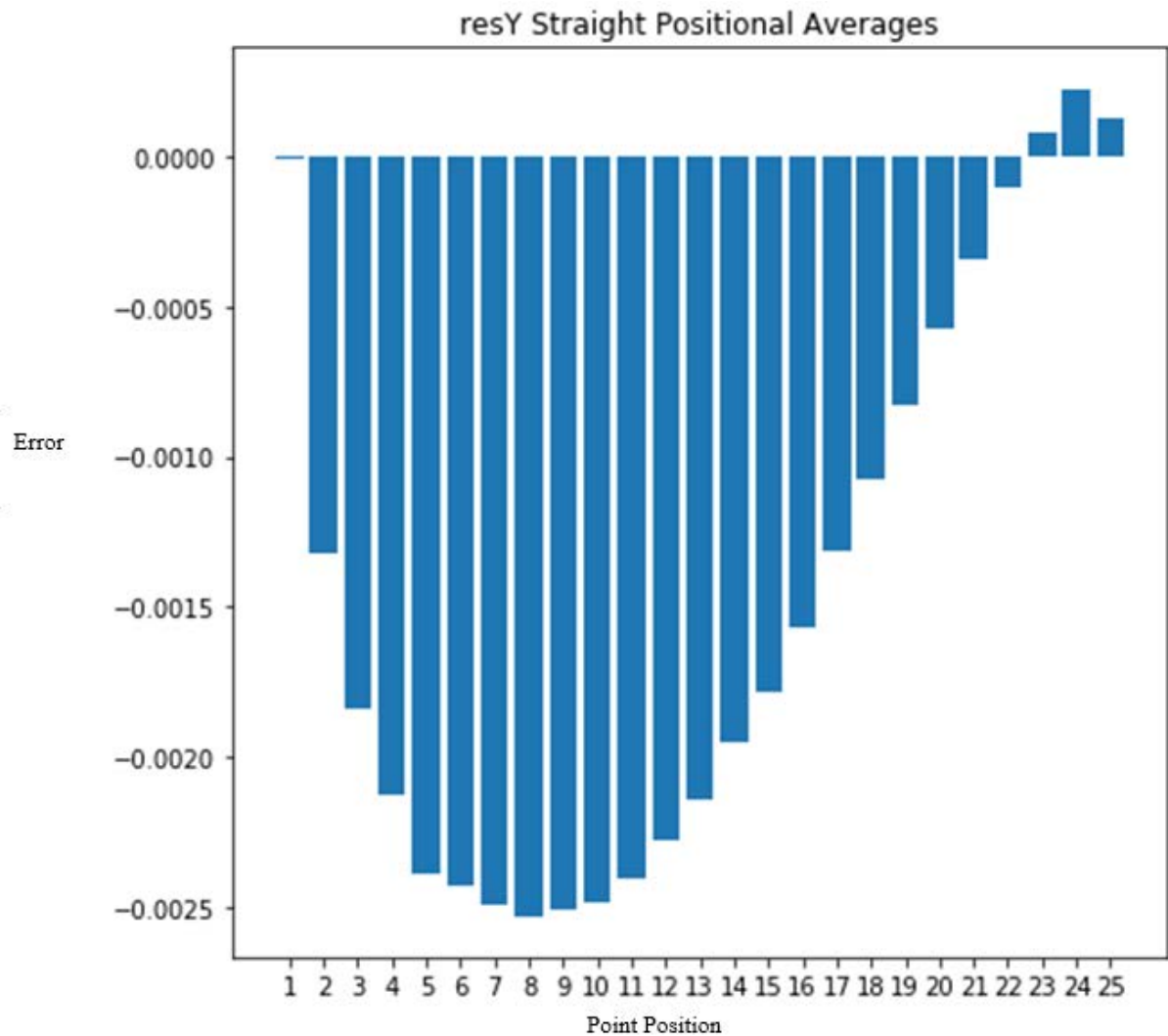
Figure 57: Data trajectory Y value residual error averages.
