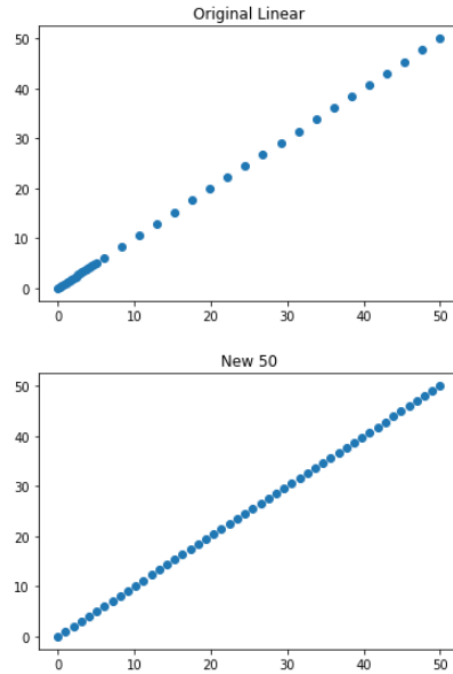
Figure 59: Interpolation example.
