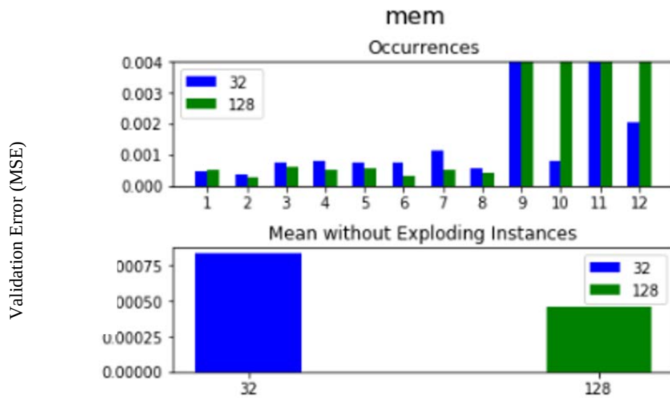
Figure 18: Capacity Comparison
