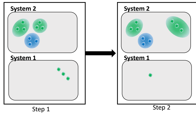
Figure 12: Revoking.
