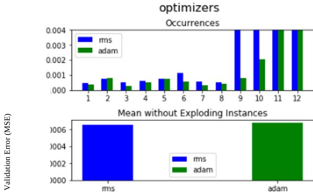
Figure 20: Optimizers Comparison
