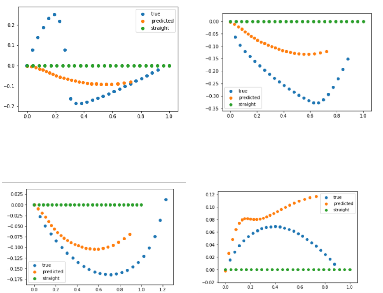
Image 18: Average predictions
