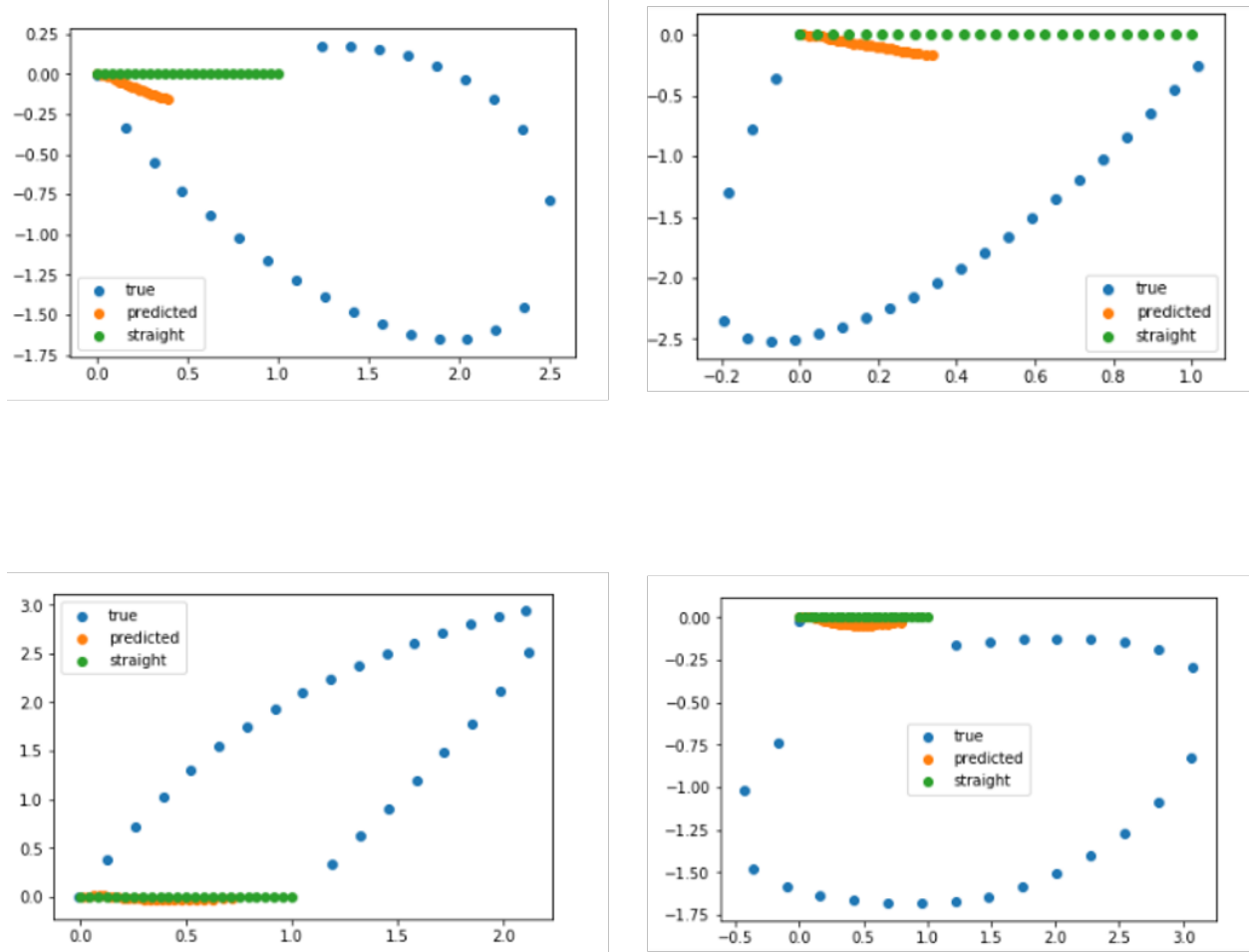
Image 19: Worst predictions
