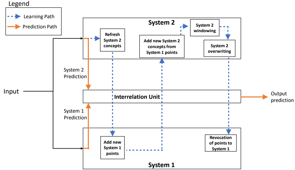
Figure 5: DPM-MN overview.
