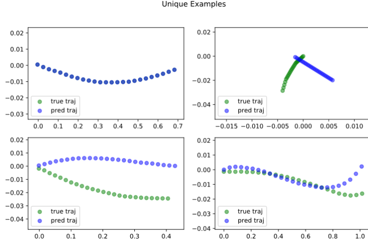
Figure 42: Unique examples.
