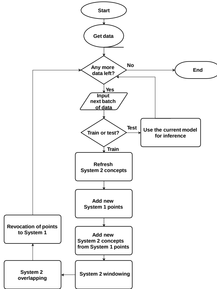
Figure 6:DPM-MN flowchart.
