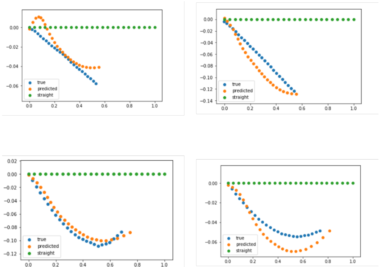
Image 17: Best predictions
