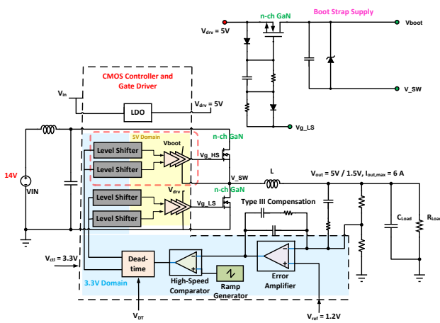
Fig. 2. Detailed block diagram of the presented hybrid CMOS/GaN buck converter.
