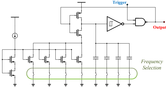
Fig. 7. Schematic of the ramp generator.
