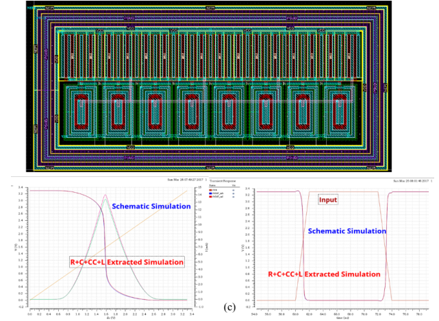
Fig. 9. ELT layout of the RHBD inverter with the transfer characteristics and transient performance showing that the extracted simulation closely matches with schematic simulation.
