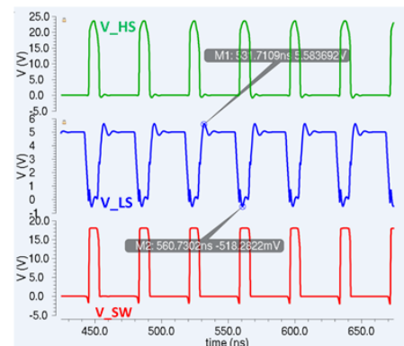
Fig. 4. Post-extracted transient simulation of the HS and LS PWM output signals.
