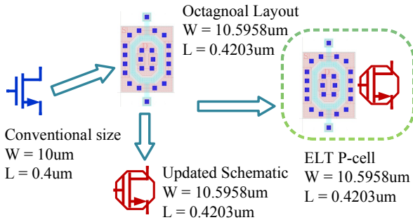
Fig. 8. Procedural flow for parameter calculation of the ELT transistors from the foundry-provided conventional (non-radhard) transistor.
