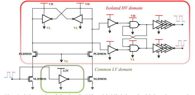
Fig. 5. Schematic of the level-shifter, highlighting the high-voltage and low-voltage domains.
