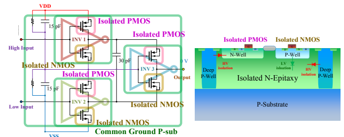
Fig. 3. Schematic of the House of Cards (HoC) cascode implementation using low voltage transistors to drive the high voltage GaN, and cross-section of the inverter with different layers for layout.
