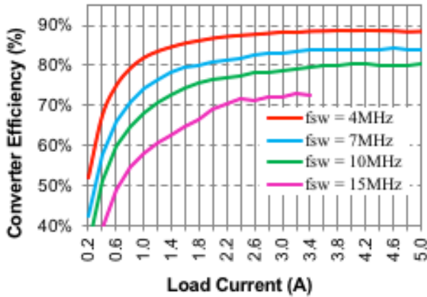
Fig. 11. Measured efficiency versus load current for a 14V input to 5V output conversion with varying switching frequencies. A switching frequency of 4MHz gives 88.6% peak converter efficiency.
