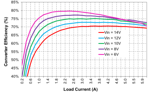
Fig. 12. Measured efficiency versus load current at 4MHz switching frequency for 1.5V output voltage and varying input voltages.
