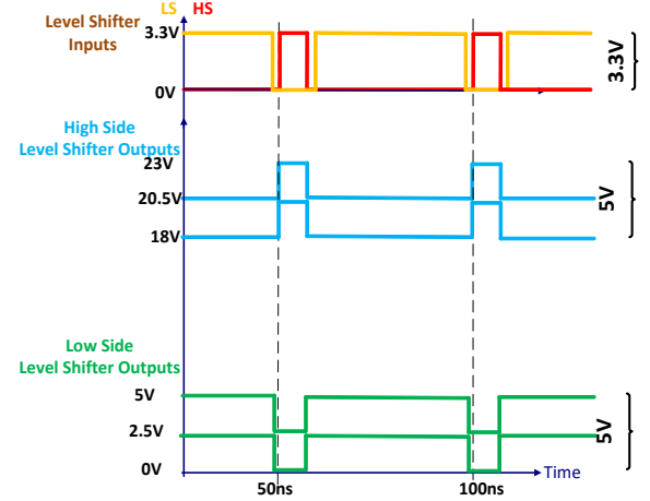
Fig. 6. Level-shifter’s timing diagram showing inputs, low-side outputs, and high-side outputs.
