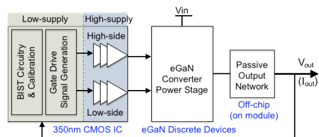
Fig. 1. Conceptual diagram illustrating hybrid converter architecture using CMOS controller and driver IC.
