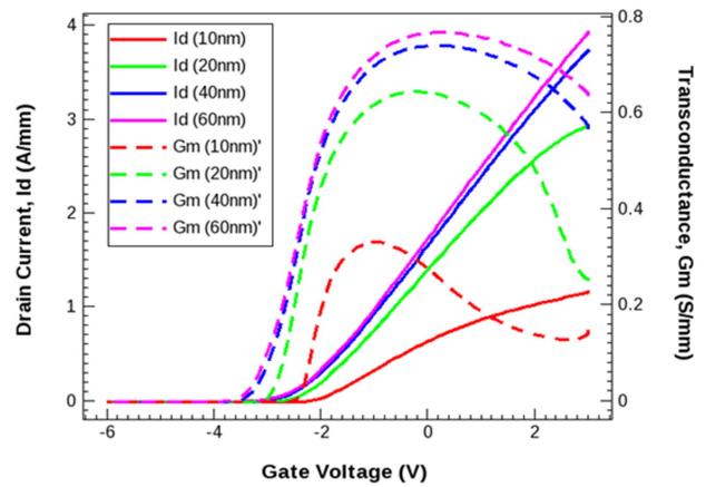
Figure 2. Simulated drain current and transconductance curves plotted vs. gate voltage for AlN/Al 0.70 Ga 0.30 N HEMT for four access region barrier thicknesses. The drain voltage is 40 V.
