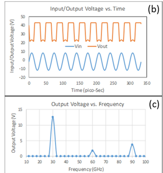
Figure 5. For simulated AlGa N -channel HEMT: (a) V_{out} vs. V_{in} transfer curve; (b) Input and output voltage waveforms; and (c) Frequency spectrum of the output voltage at 30 dBm input power.
