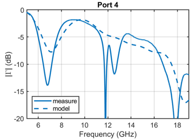
Fig. 3 – Reflection coefficient of fragmented aperture antenna as modeled and measured from 6 to 18 GHz.
