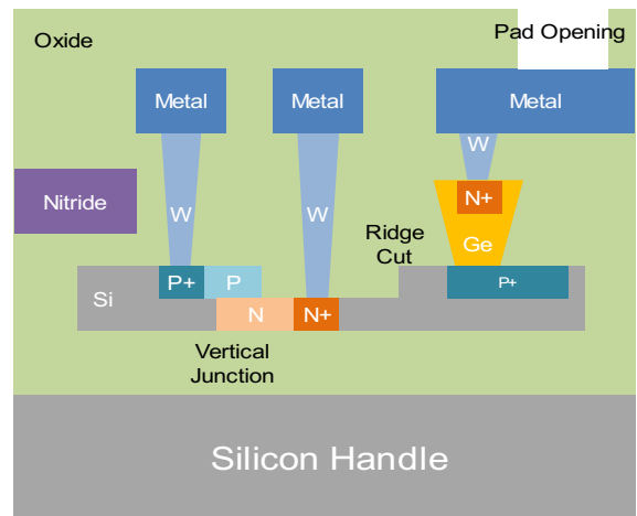
FIGURE 3. Silicon Photonics platform device schematic.
