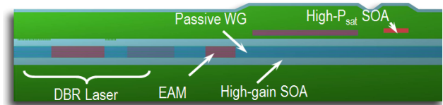
FIGURE 6. Depiction of the cross-section of an example photonic integrated circuit which shows the various regions tailored for specific functions of a particular device.
