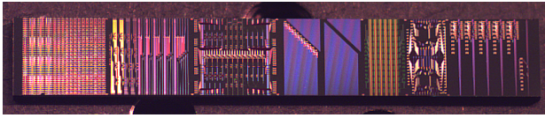
FIGURE 5. A set of devices from a Silicon Photonics multi-project wafer run.
