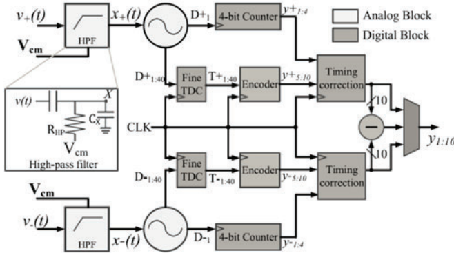
Fig. 5. Architecture of VCO-based ADC from KGD.
