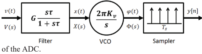
Fig. 4. VCO-Based ADC conceptual diagram.
