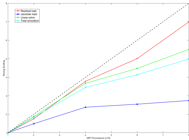
Fig. 9. 1M memory circuit strong scaling
