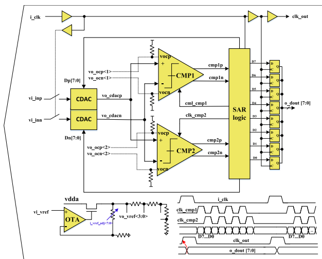
Fig. 2. A simplified block diagram of a sub-ADC.
