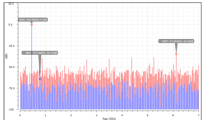
Fig. 3. The ADC output spectrum before (red) and after (blue) calibration.
