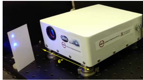
Fig 4. An early Phase 2 prototype compact DUV laser was demonstrated at the DARPA D-60 event. Seen on left are the 232nm (top) and 464nm beams. cavity length to make it resonant for blue beam wavelength, and by using a novel segmented walk-off compensated BBO crystal that will reduce the walk off during fourth harmonic conversion. Work is in progress to implement these two steps and the resulting improvements will be reported.
