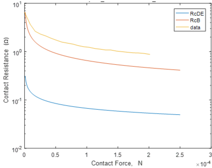
Figure 40. Resistance of the micro-contact for forces up to 200 \mu N after 10 cycles compared to models for ballistic electron transport with a Knudsen of 10, labeled as RcB and for diffusive electron transport labeled as RcDE.
