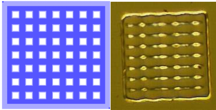
Figure 39. Micro-contact design in L-Edit specified by DOE run #4 and the resulting design after fabrication.
