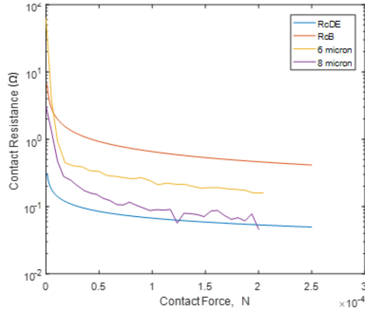
Figure 67. Resistance of the micro-contacts for forces up to 200 \mu N after a million cycles.
