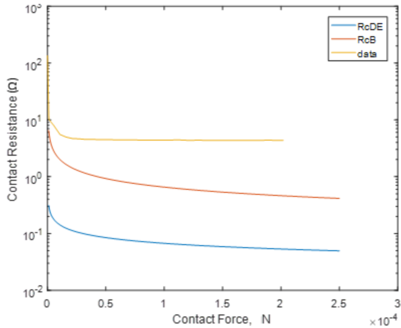
Figure 49. Contact resistance for forces up to 200 \mu N after the millionth cycle.
