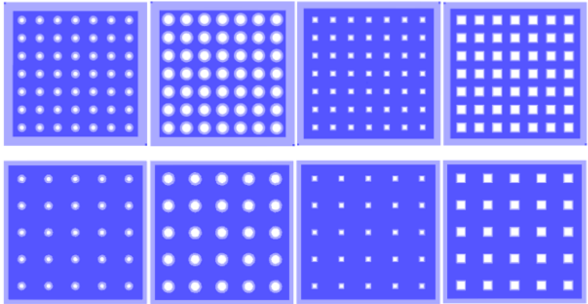
Figure 20. L-Edit designs for the 2^4 factorial experiment. Each design is 32\text{ }\mu\text{m} by 32\text{ }\mu\text{m} . The white denotes the highest point of the micro-contact and the dark blue denotes the lowest point of the contact.
