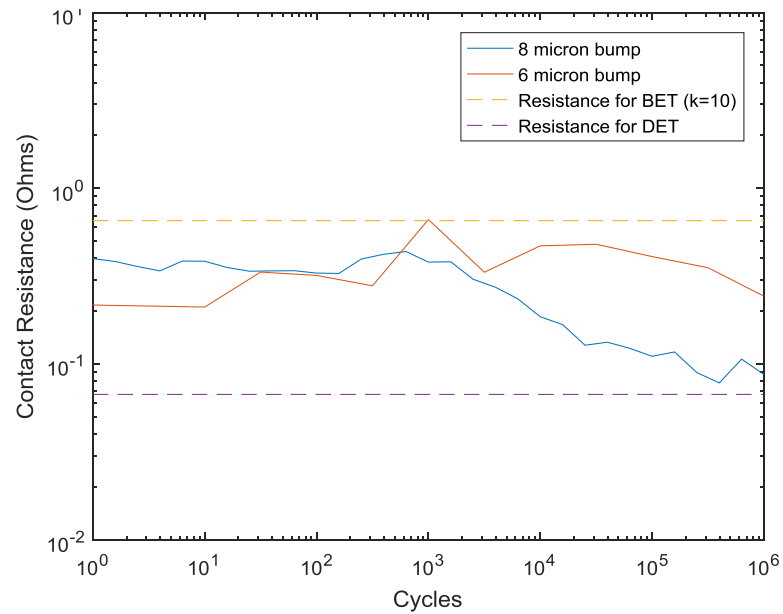
Figure 68. Comparison of the resistance measured when 100 \mu N is applied between a contact with a 6 \mu m upper bump radius and an 8 \mu m upper bump radius.
