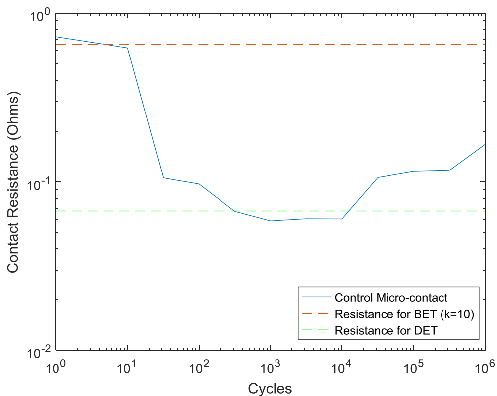
Figure 56. Resistance of the micro-contact with 100 \mu N applied to the beam taken at test points throughout testing. BET stands for ballistic electron transport and DET stands for diffusive electron transport.
