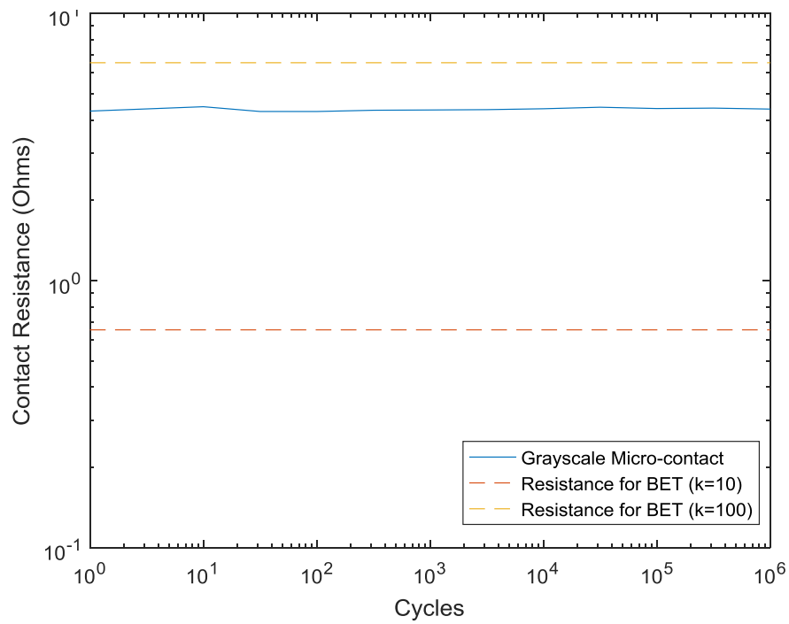
Figure 50. Contact resistance measured while 100 \mu N was applied to the beam taken at test points throughout testing.
