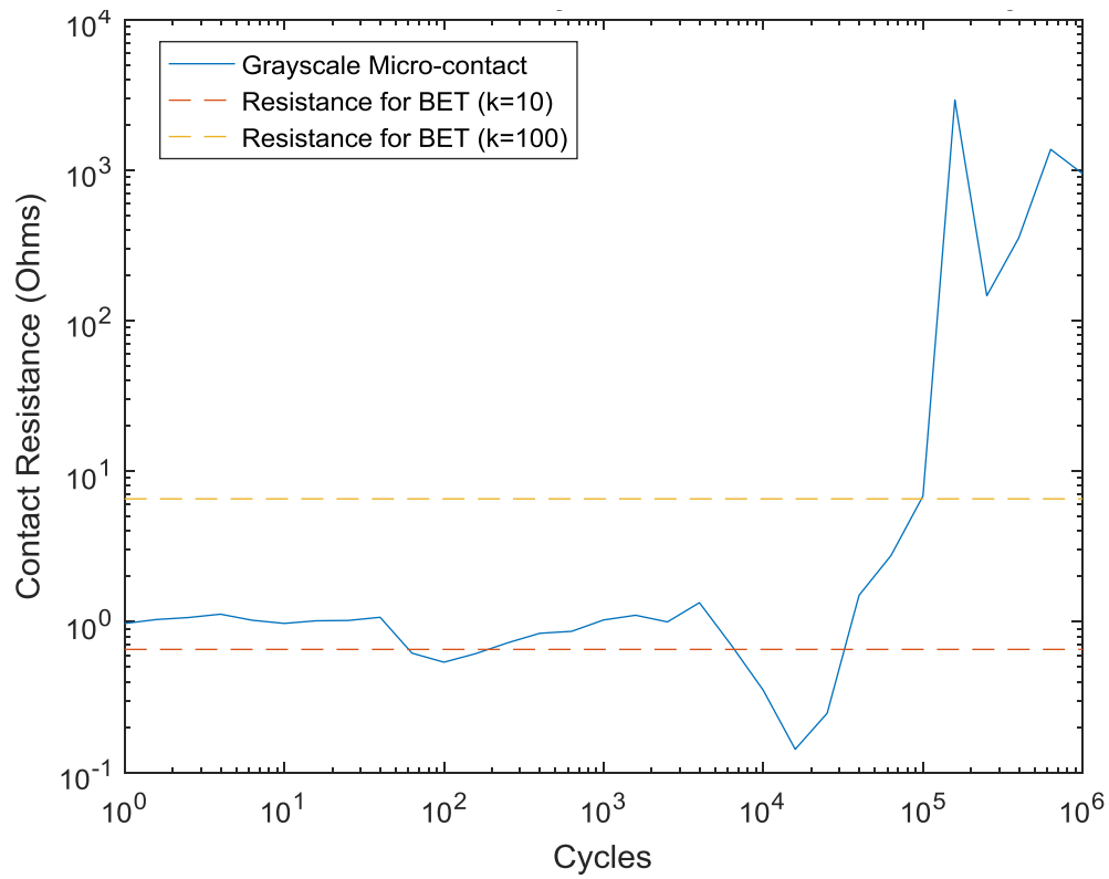
Figure 46. Resistance of the micro-contact while 100 \mu N is applied taken at test points spread out over the duration of testing. The sharp increase in resistance near the end of testing is an indicator of a failure mechanism.
