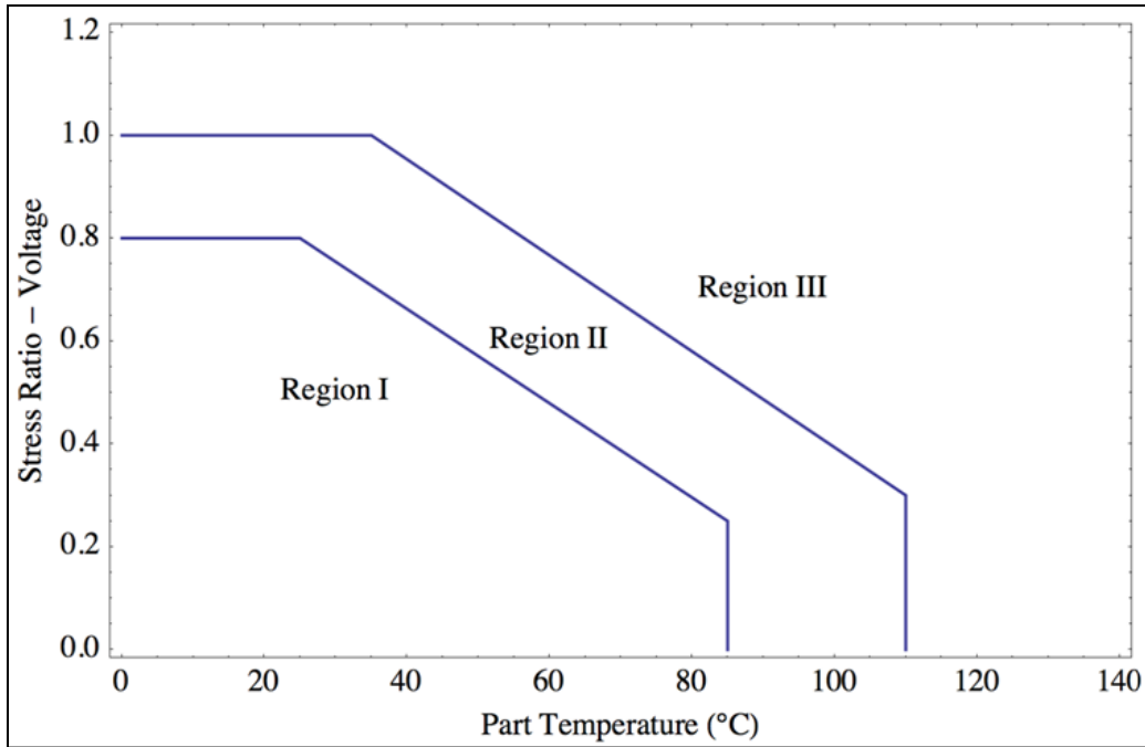
Figure C-4. Mica (CMS)
