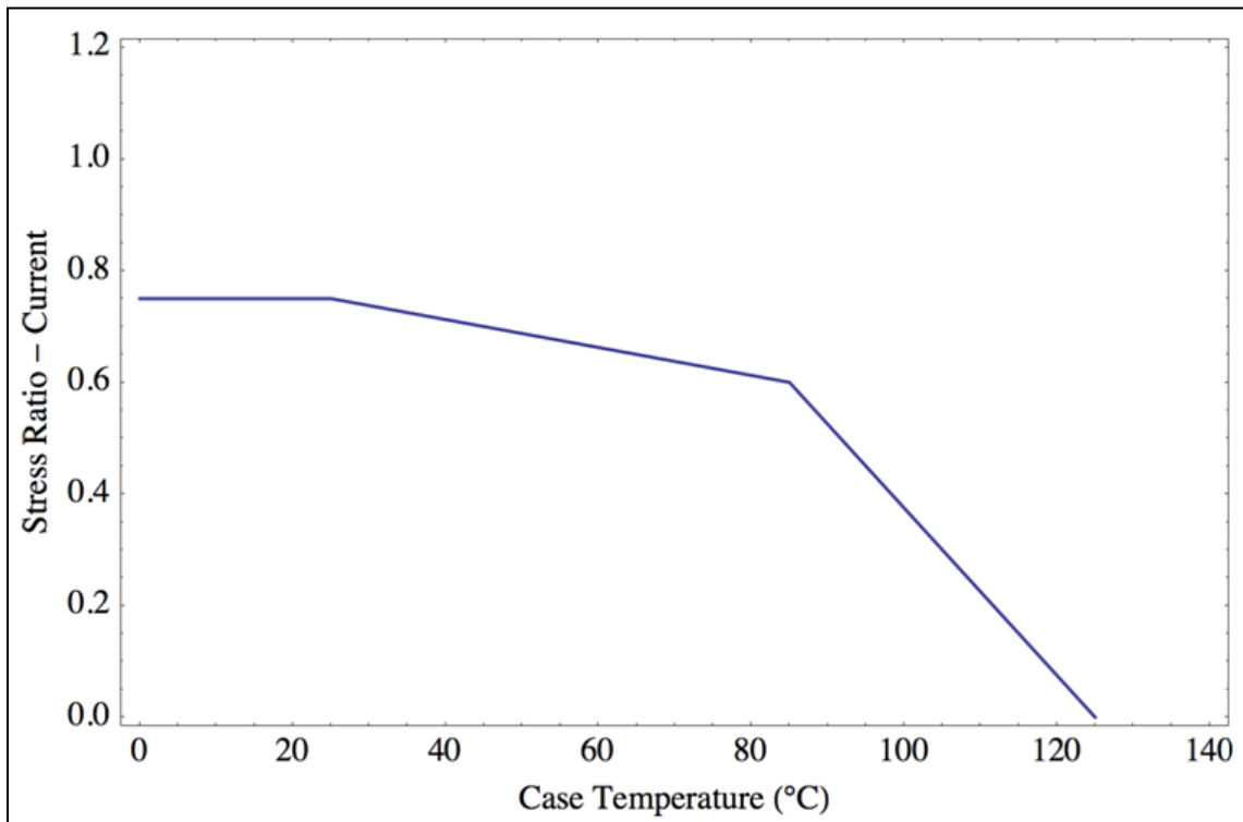
Figure C-8. Solid-Body Fuses
