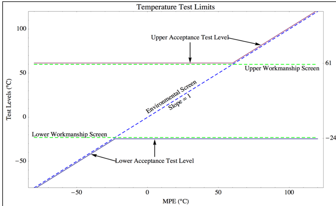
Figure 4-3. Acceptance Thermal Cycle Temperatures - Non-Ordinance
