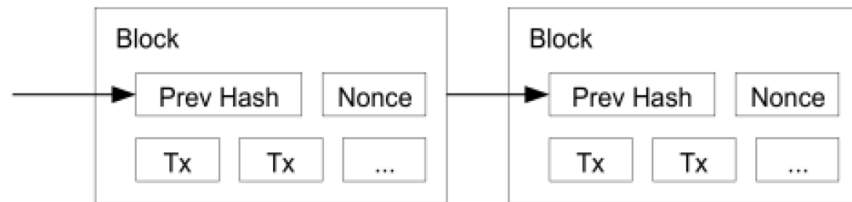
Figure 4. Bitcoin Block Structure [16]
