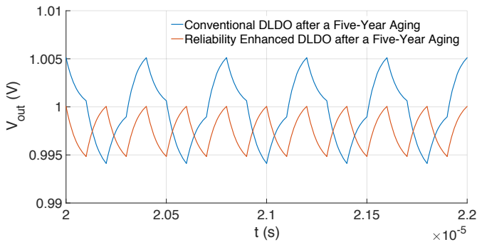
Fig. 5. Output voltage ripple comparison between a conventional DLDO with LCO mitigation and the reliability enhanced DLDO with LCO mitigation after a five-year aging period.
