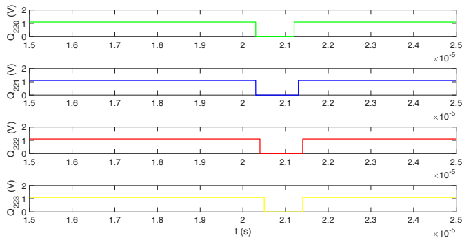
Fig. 4. Representative gate signals of the reliability enhanced DLDO with LCO mitigation.
