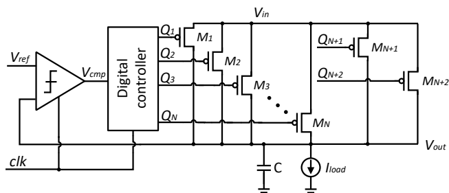
Fig. 1. Schematic of DLDO with LCO mitigation.
