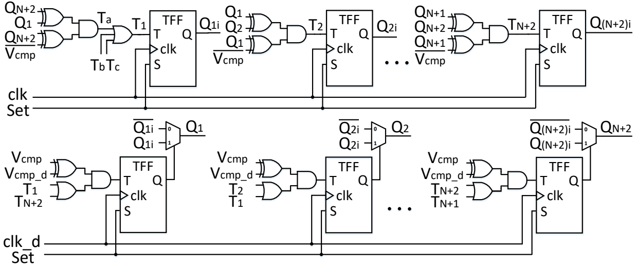
Fig. 3. Proposed N + 2 bit unidirectional controller for reliability enhanced on-chip DLDO with LCO mitigation.
