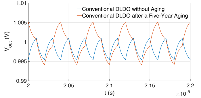
Fig. 2. Output voltage ripple of a conventional DLDO with LCO mitigation technique before and after a five-year aging period.
