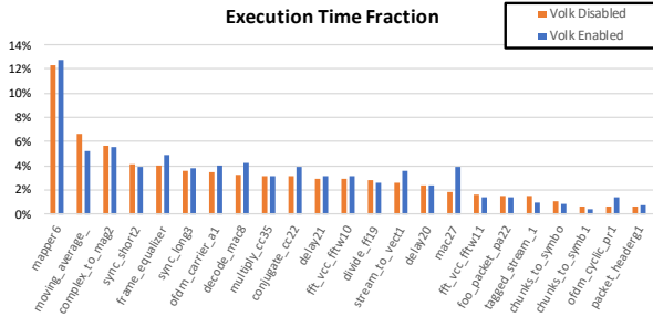
Fig. 7: Execution time fraction of GNU Radio/802.11p on x86.
