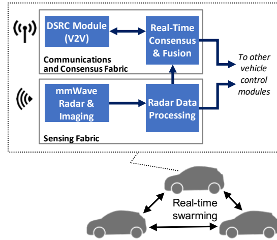
Fig. 4: Swarm-based sensor fusion in connected/autonomous vehicles as part of our DARPA-sponsored EPOCHS project.
