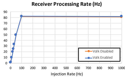
Fig. 8: Processing rate of GNU Radio/802.11p receiver on x86.
