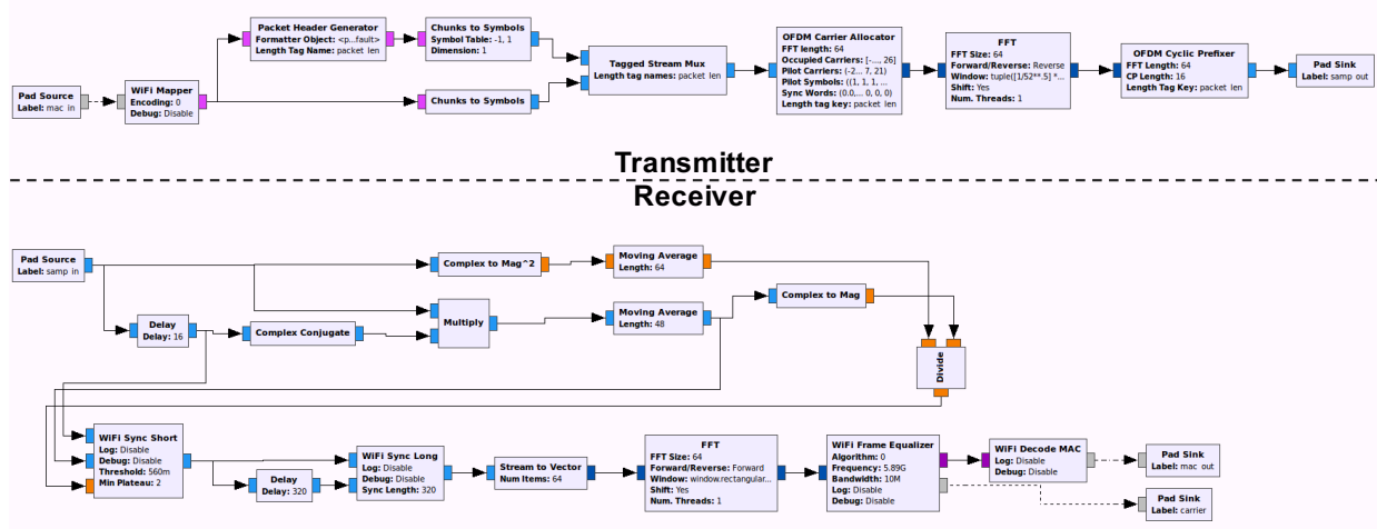
Fig. 6: GNU Radio-based 802.11p transceiver flowgraph [12], [13].
