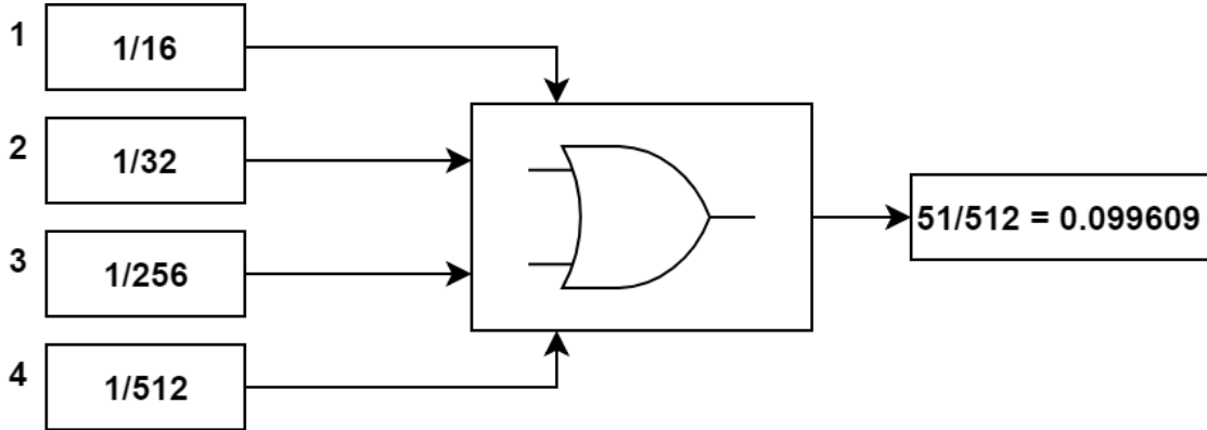
Figure 18. Linear Feedback Shift Register Example, 10% Desired Chip Inversion.
