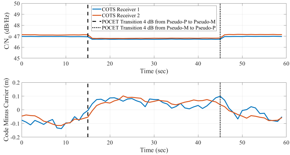
Figure 25. Alternating Transitions of 4 dB from P to M Signals
