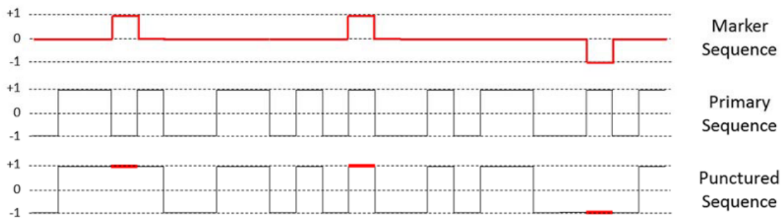
Figure 8. Puncturing Example (From [1], Used With Permission)
