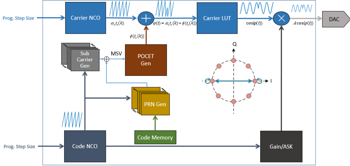
Figure 9. GWPP Architecture
