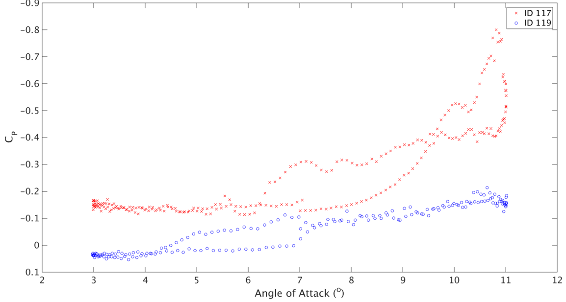
Figure 4.15: Comparison of C_P values at pressure station 3, at 70.0% chord for runs cases ID117 (5.7 Hz) and ID119 (7.6 Hz)
