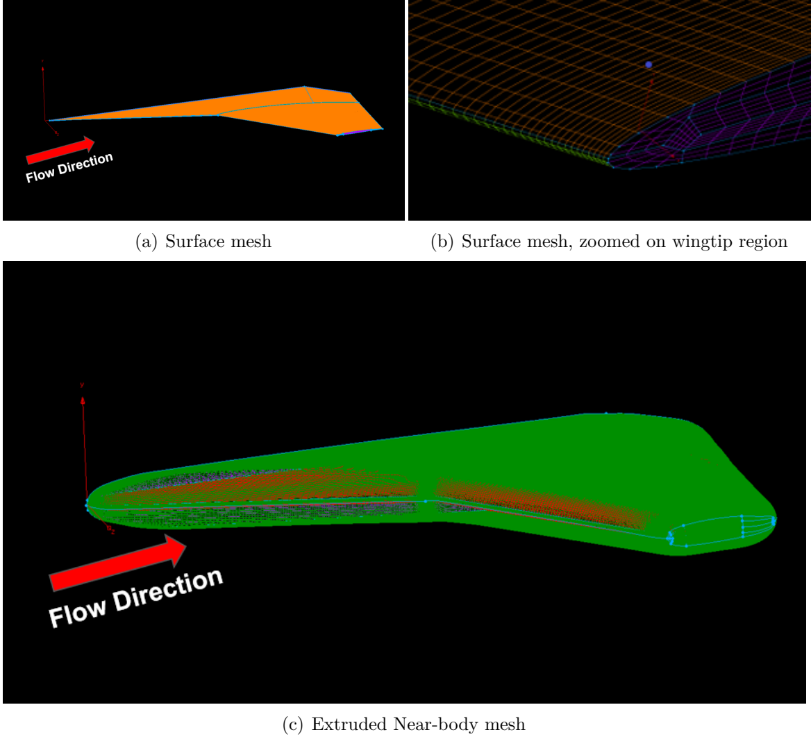
Figure 3.3: Two stages of creating the near-body mesh
