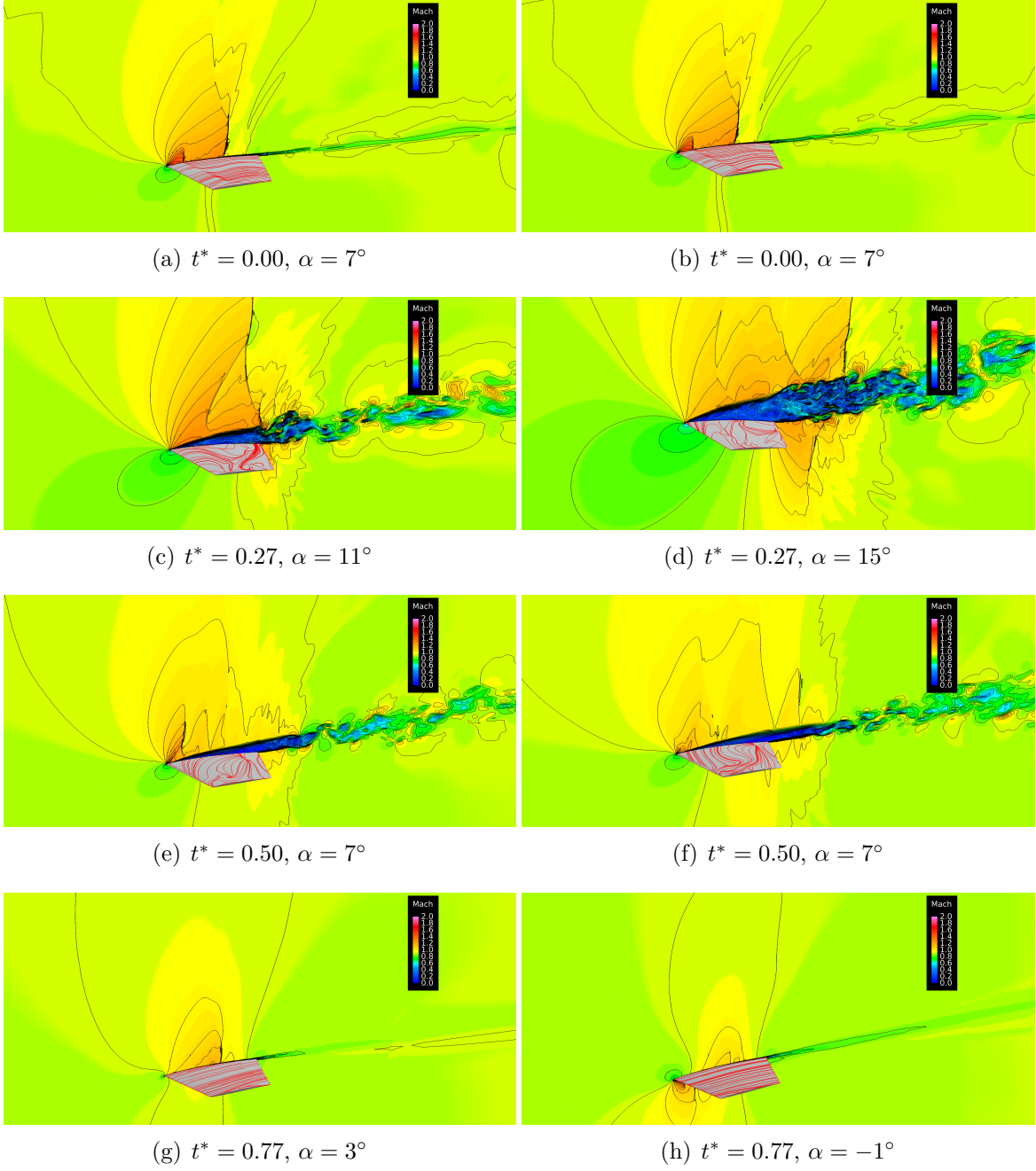
Figure 4.9: Mach contours comparison at pressure station three with a Mach of 0.9, trim of 7^\circ , frequency of 7.6 Hz. The left column used an amplitude of 4^\circ while the right used 8^\circ
