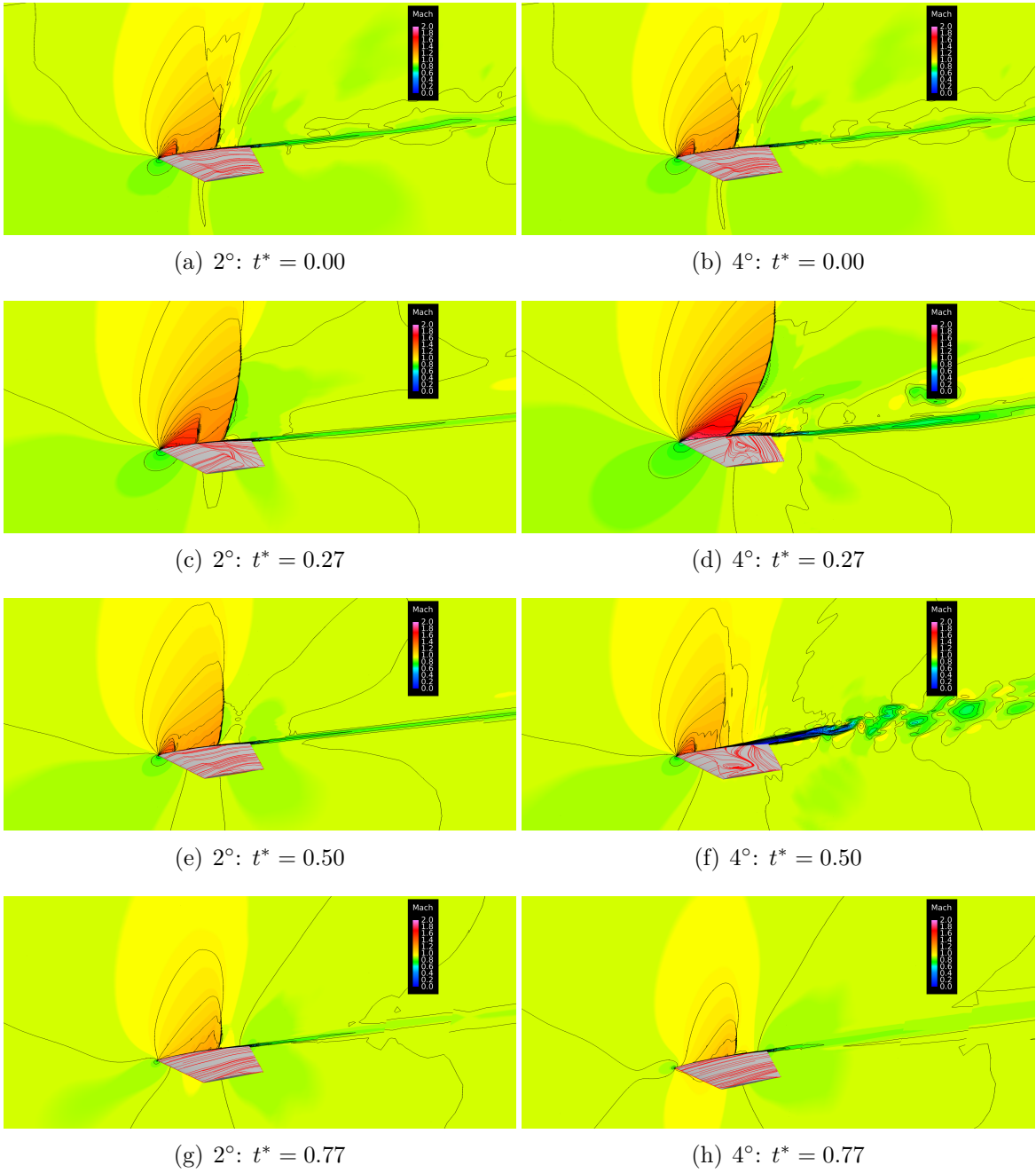
Figure 4.7: Mach contours comparison at pressure station three with a Mach of 0.9, trim of 4^\circ , frequency of 7.6 Hz and varying oscillation amplitude
