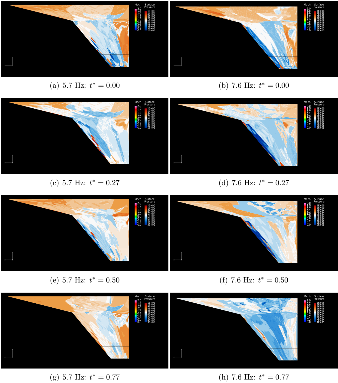
Figure 4.16: Surface Pressure comparison at a Mach of 0.9, trim of 7^\circ , amplitude of 4^\circ and varying frequency
