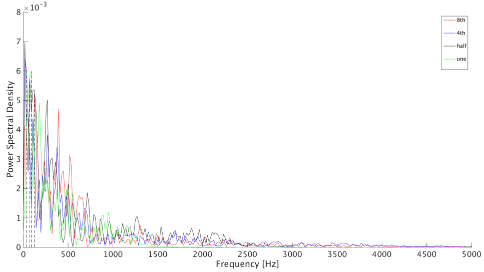
(a) PSD of unsteady C_P on Medium grid with four time steps
