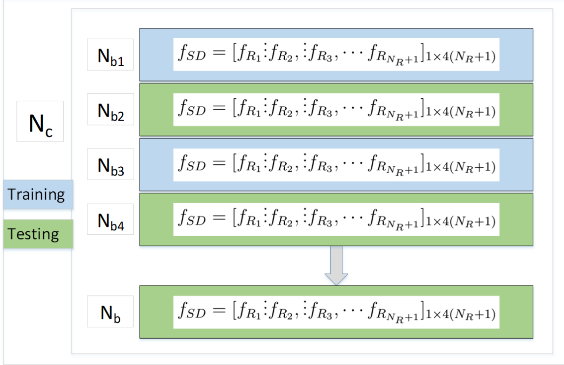
Figure 15. Training and Testing Data Sets Chosen In An Interleaving Pattern
