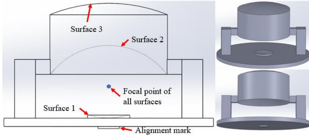
Figure 16. Confocal Surfaced Double Cavity FPI Fiber Tip Sensor
