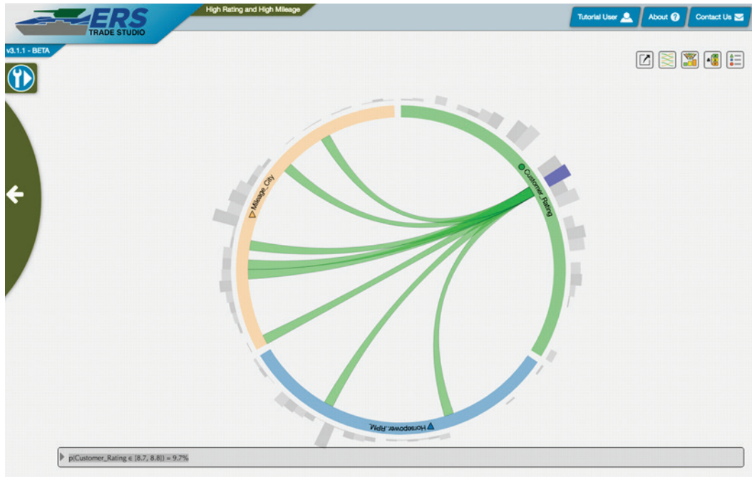
Figure 43. Single bin selected.
