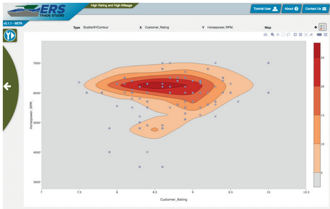
Figure 68. Explore Tool ScatterXYContour view.
