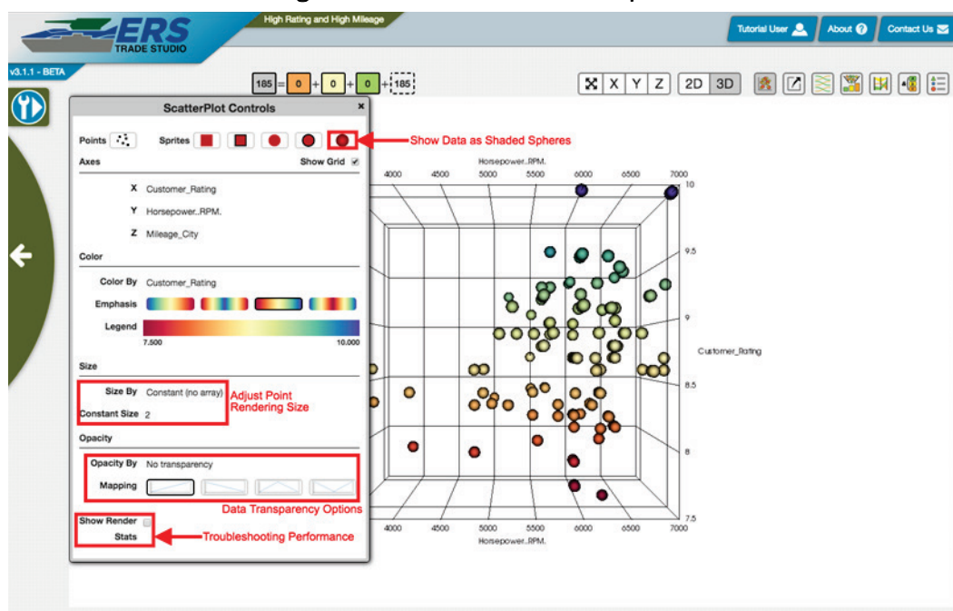
Figure 47. Plot Tool – additional options.
