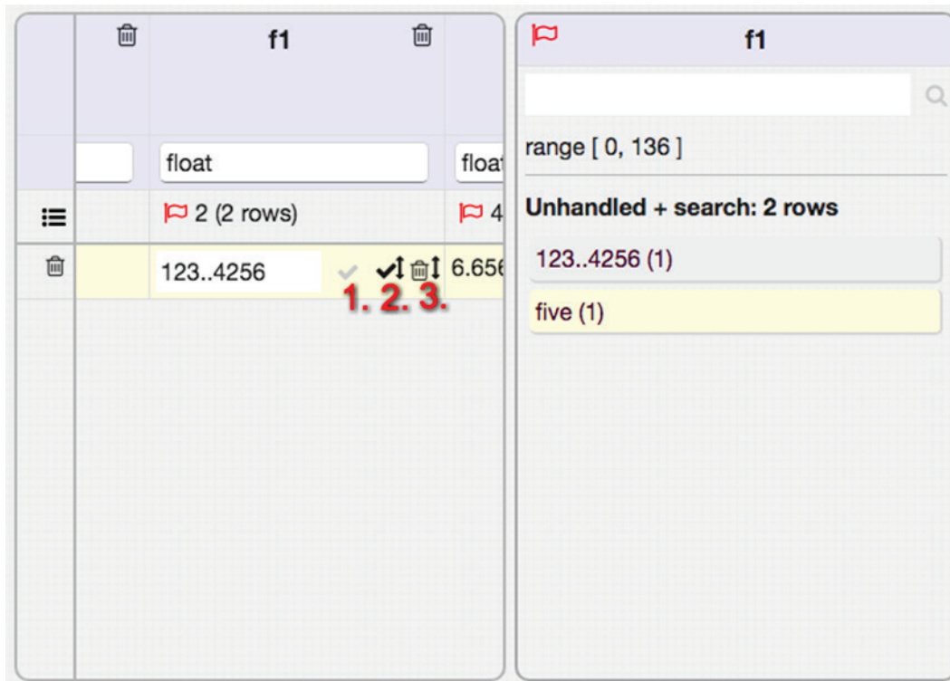
Figure 19. Data cleaner editing values.
