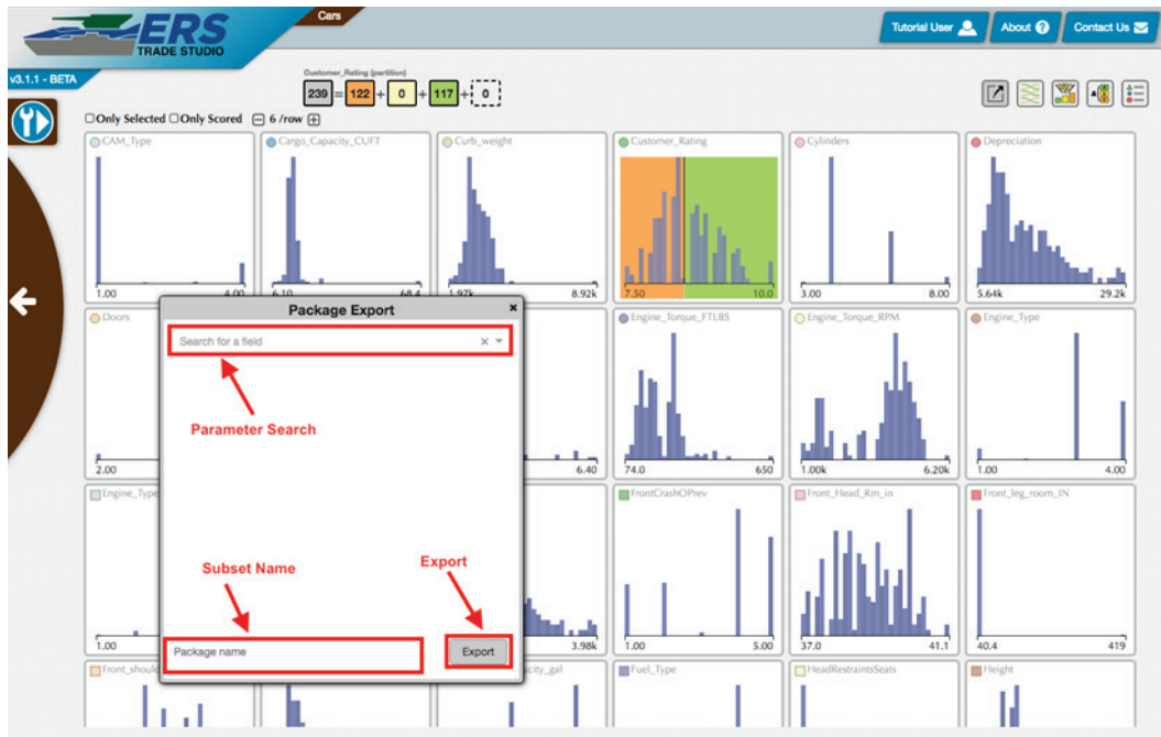
Figure 33. Export Package View.
