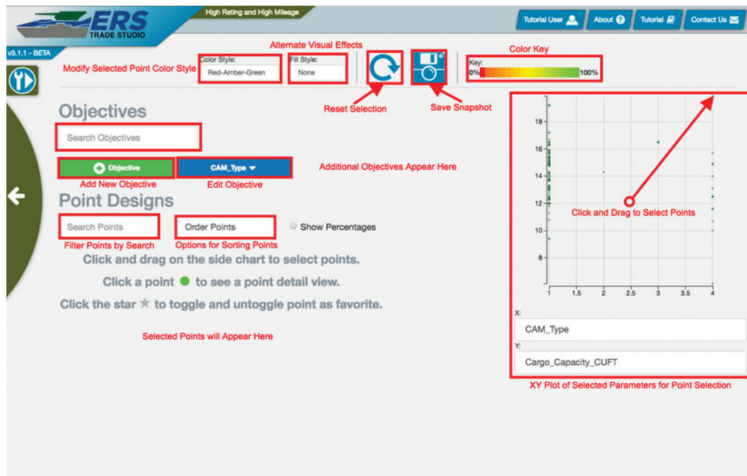
Figure 54. Select tool home page.
