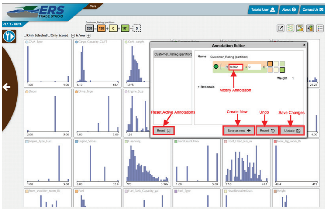
Figure 28. Annotation Editor – partition.
