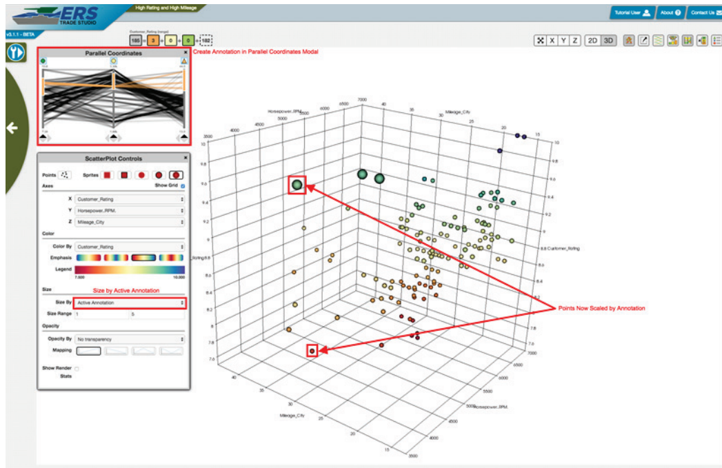
Figure 48. Plot Tool – Compare Tool annotations.
