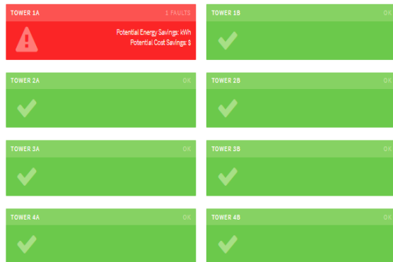
Figure 11. Screen shot of the cycling fault detection results overview in the PlantInsight tool for a time period during which a tower fan cycling fault was detected
