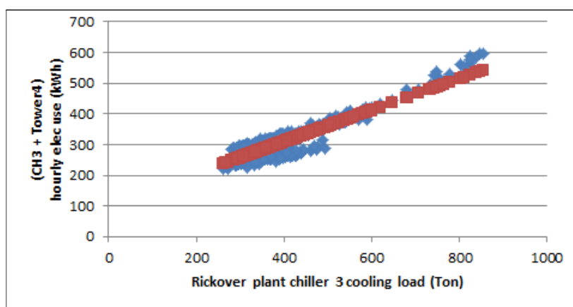
Figure 29. Baseline energy data: metered (blue) vs. modeled (red)
