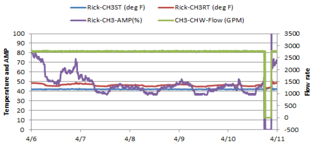
Figure 24. Operational data for Rickover Chiller 3: April 6–10, 2017
