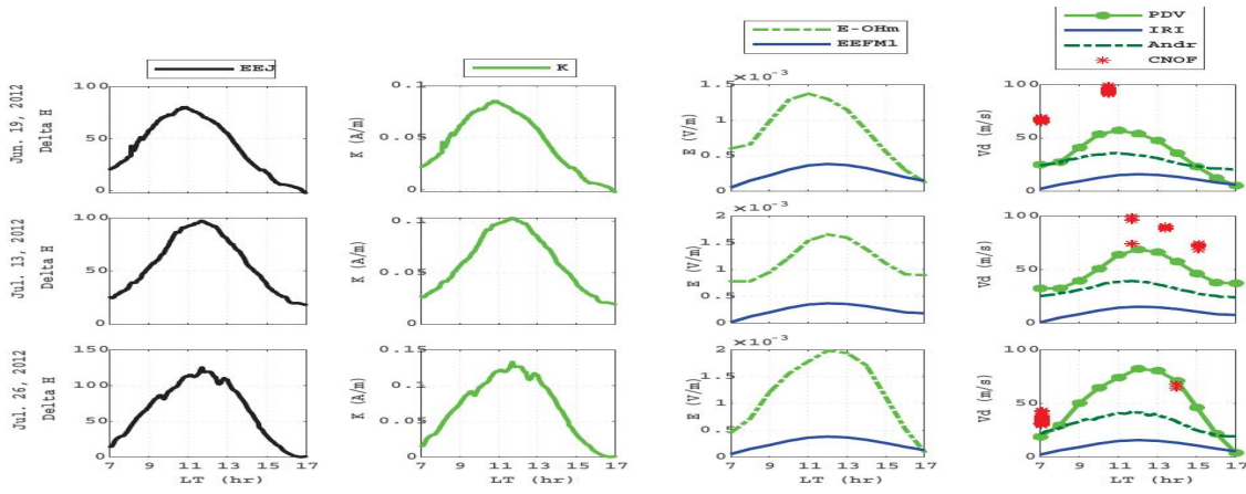
Figure 14: Daytime EEJ, estimated sheet current density, E-field and vertical ion drift velocity over Jicamarca Radio Observatory, Peru on 19 June 13 and 26 2012.
