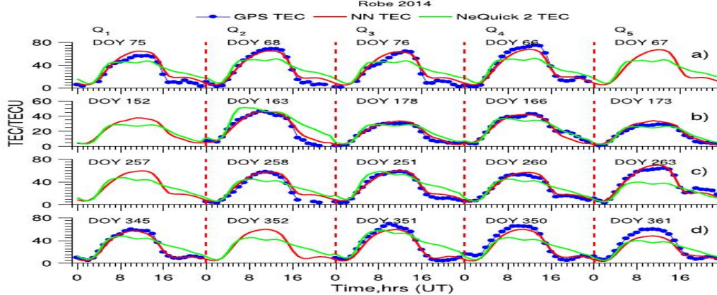
Figure 13: Diurnal variation of NN and NeQuick modeled and GPS observed TEC in the year 2014.
