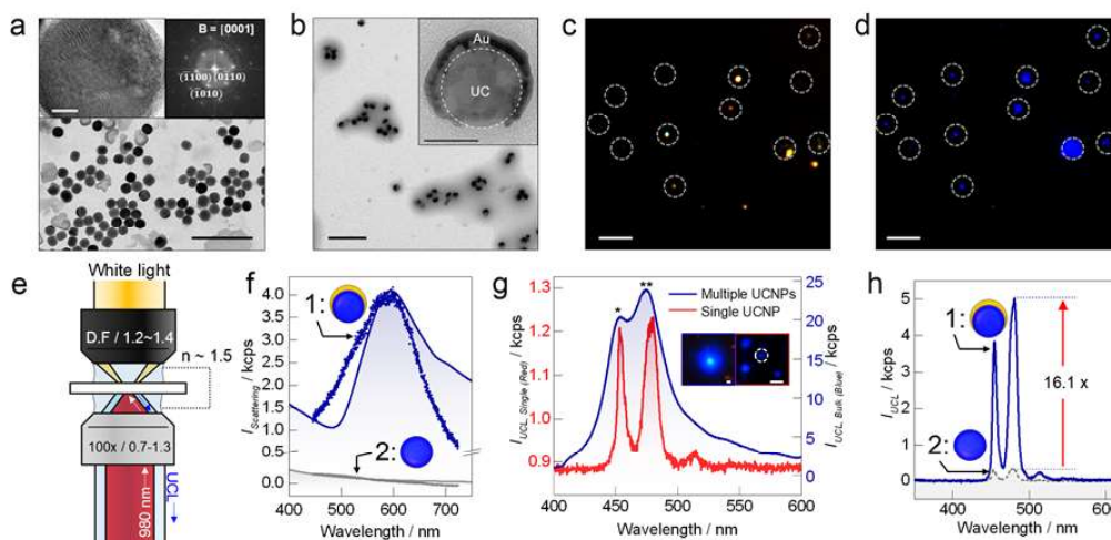
Figure 32. Optimization of nanofocusing of excitation light. (a) Transmission electron microscopy (TEM) image of upconversion nanoparticles (UCs; NaYF 4 :Yb 3+ , Tm 3+ ) (Scalebar:100nm). Inset is a high-resolution TEM image of a UC (Scalebar:10nm) with a selected area electron diffraction (SAED) pattern. (b) TEM image of ANAUs in low magnification (Scale bar: 1 μm) and high magnification (inset; scale bar: 50 nm). (c-d) Correlated image of (c) dark-field scattering and (d) frequency upconverted emission of ANAUs (Scale bar: 10 μm). (e) Schematic diagram for optical microscopy setup for correlated measurement of dark-field scattering and frequency upconverted emission. (f) Simulated scattering cross-section (line) and dark-field scattered spectrum of an ANAU (number 1, blue) and UC (number 2, gray). (g) Frequency upconverted emission spectrum of single ANAU (red) and ensemble averaged ANAU powder (blue). The inset shows CCD images obtained from each sample (Scale bar at left: 10 μm, right: 1 μm). (h) Representative frequency upconverted emission spectrum of an ANAU (number 1) and UC (number 2).
