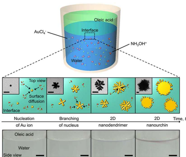
Figure 2. Schematic representation and time-resolved optical images of an oleic acid/water interface for the synthesis of two-dimensional gold nanoparticles
