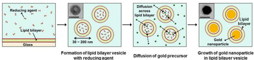
Figure 12. Schematic illustration of the synthesis of gold nanoparticles in lipid bilayer vesicle
