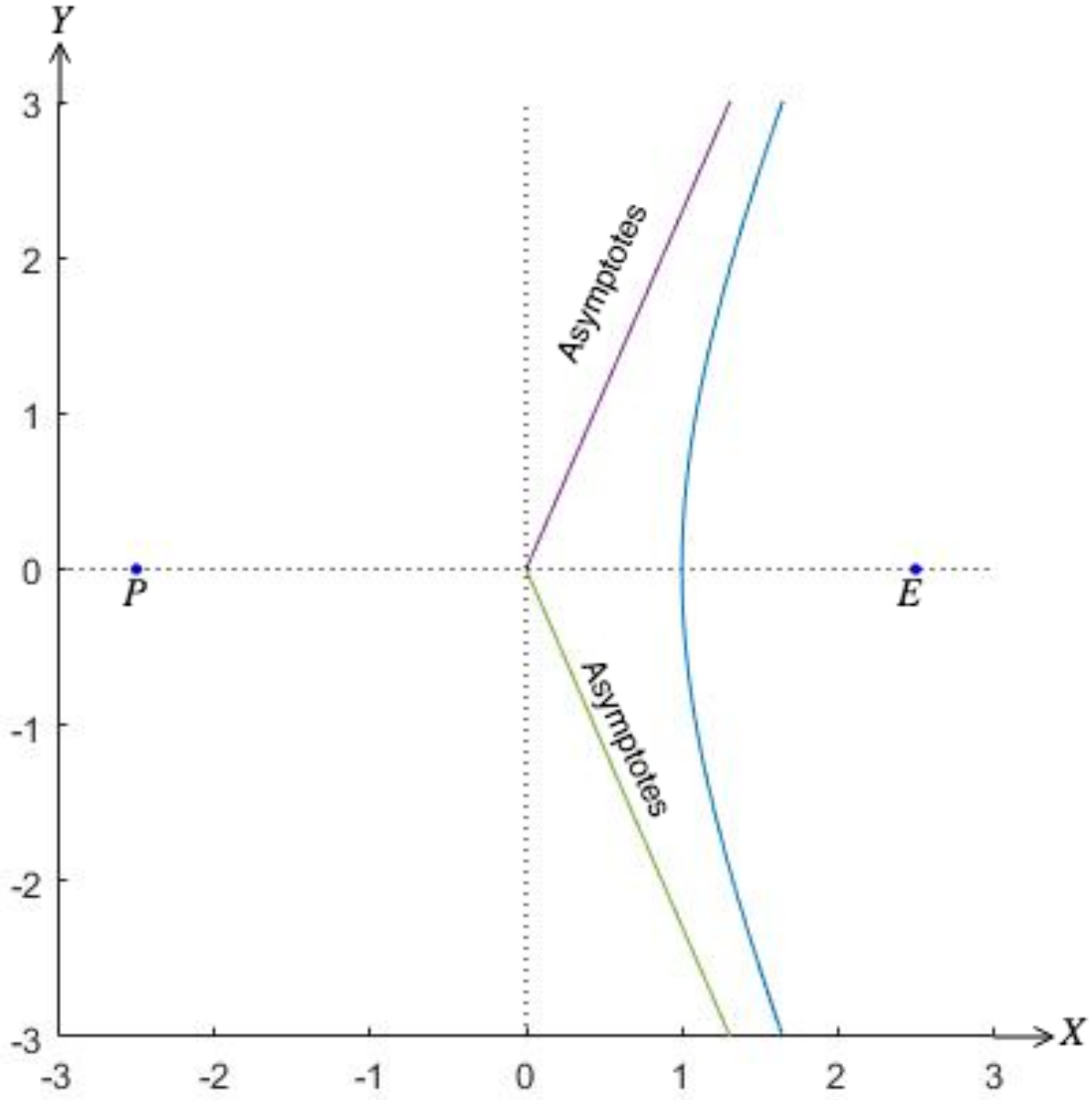
Figure 6: The Hyperbola is the BSR of E
