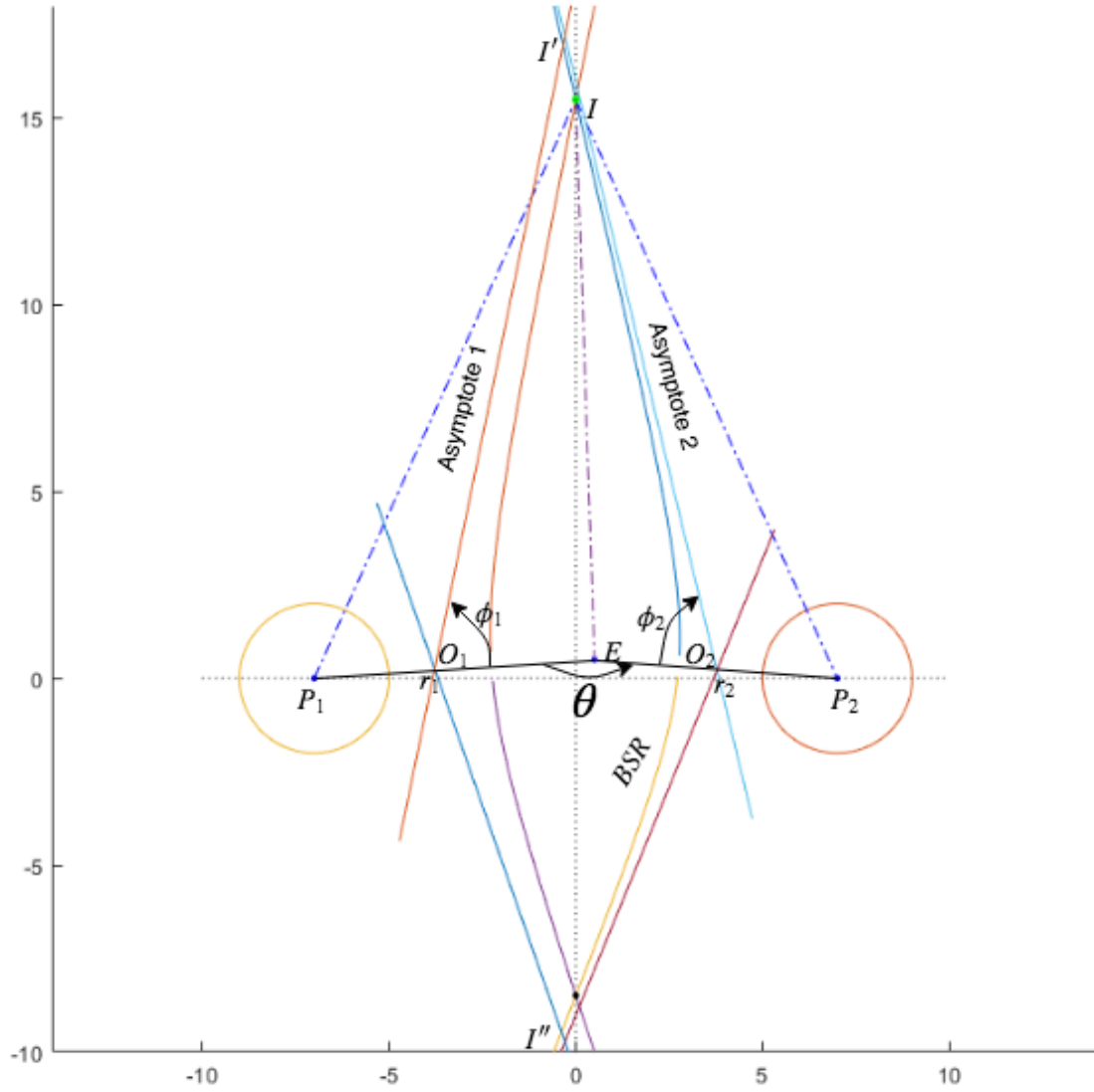
Figure 21: Quadrilateral Formed by Intersecting Asymptotes
