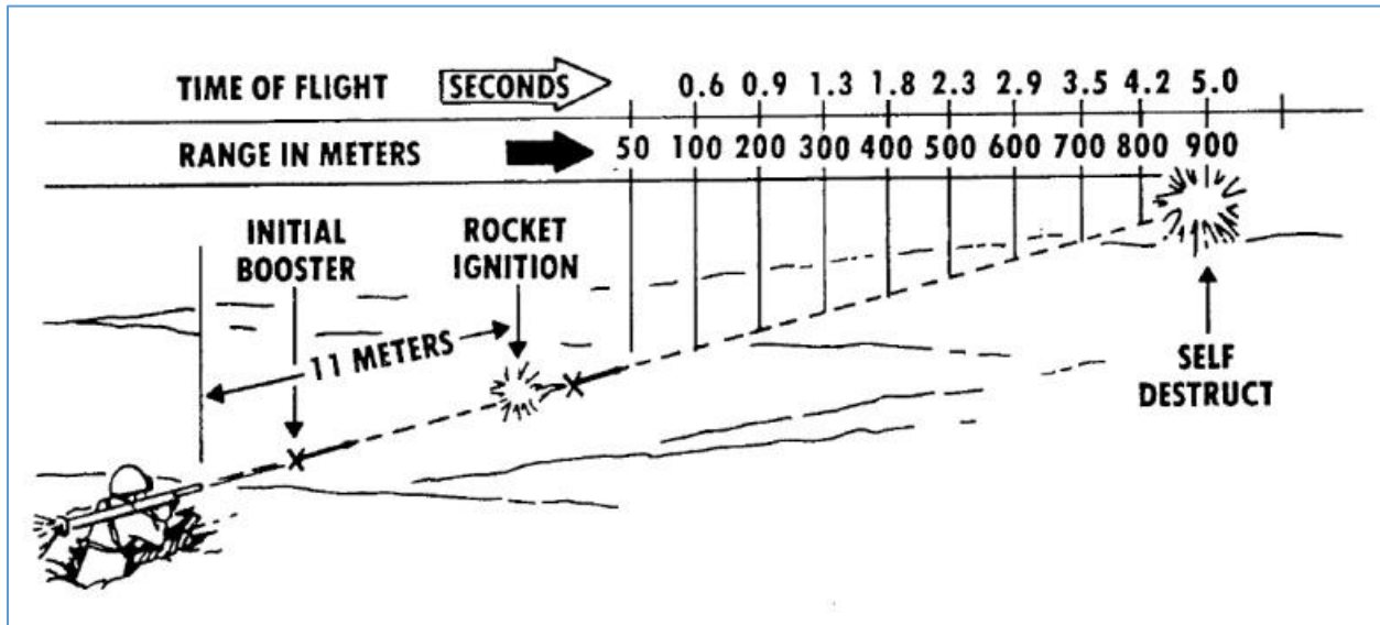
Figure 3. Launcher sequence
