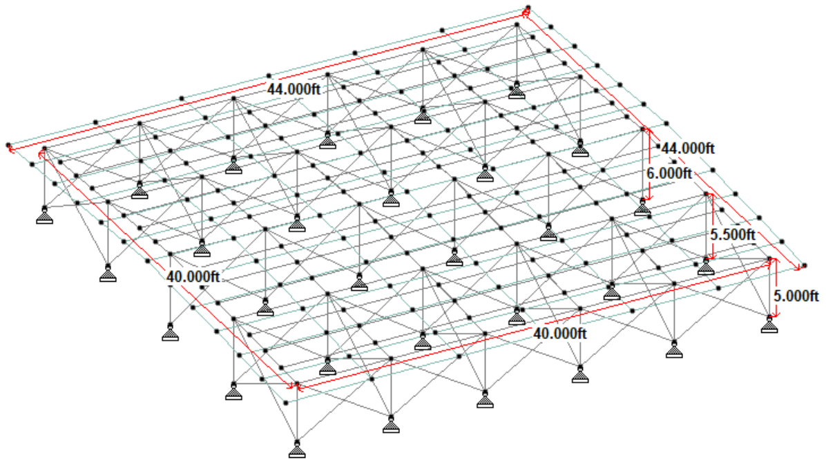
Figure 13. 40' x 40' Isometric View
