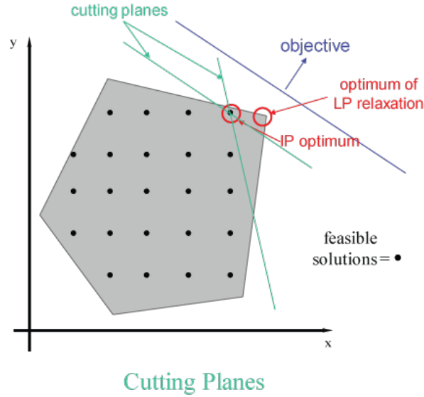
Figure 4. Cutting Plane [3]
