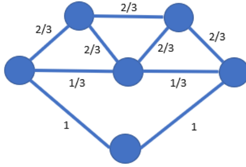
Figure 3. TSP Relaxation Solution
