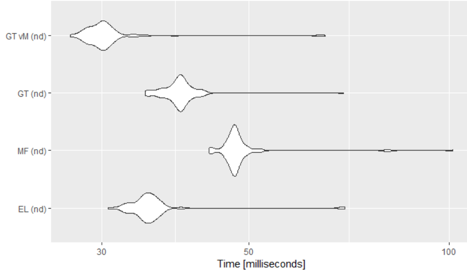
Figure 28. Microbench Output Plot
