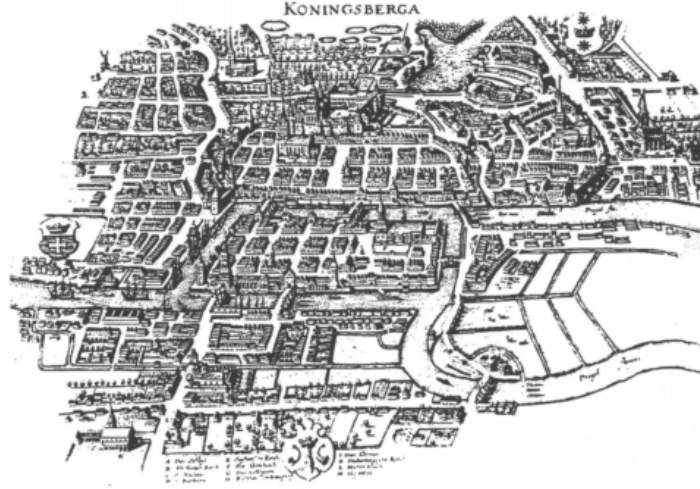
Figure 1. Königsberg Bridges [1]
