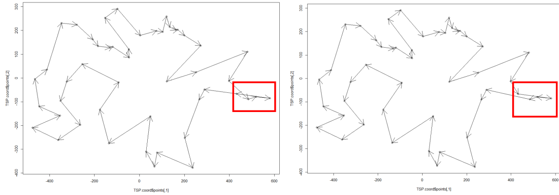
Figure 40. gr48 Optimal Tours
