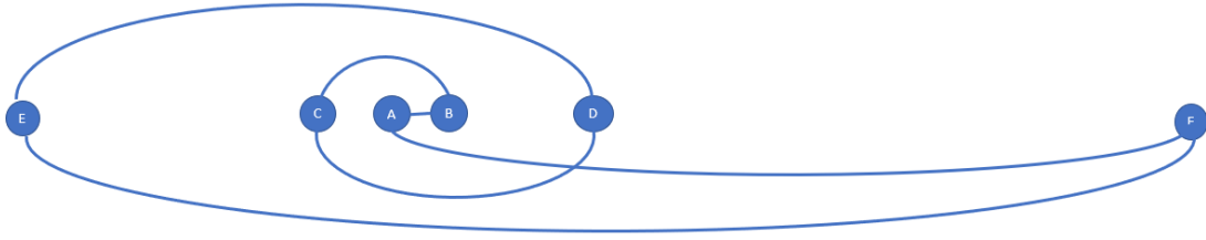
Figure 5. Greedy Worst Solution Example
