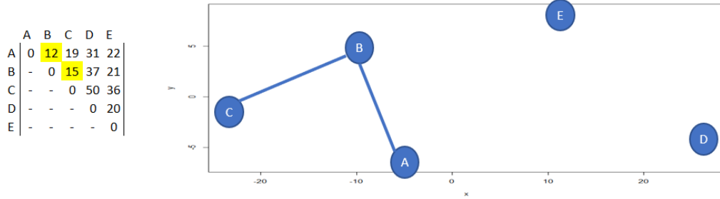
Figure 6. Greedy Subtour 1
