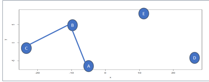
Figure 12. MF Subtour 2
