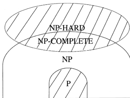
Figure 2. Computational Complexity [2]
