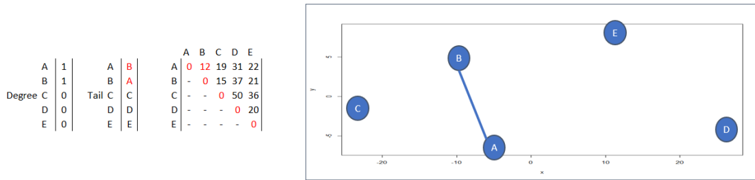
Figure 11. MF Subtour 1
