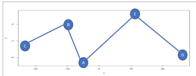
Figure 13. MF Subtour 3
