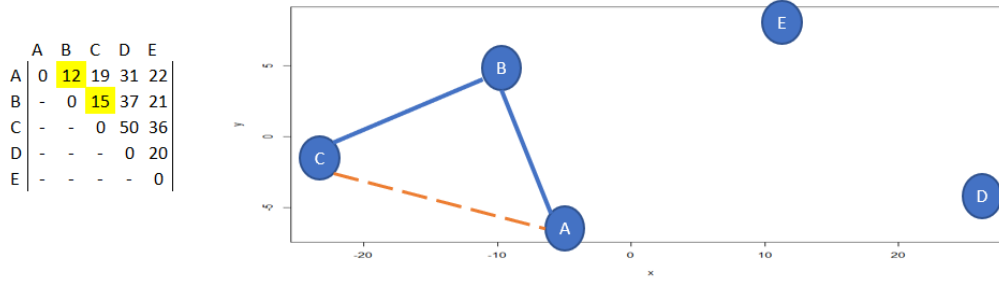
Figure 7. Greedy Subtour 2
