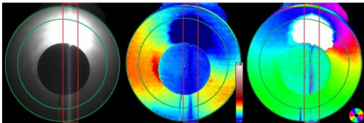
Figure 4. Polarization image captured with a 185° fish-eye lens. Left: intensity, middle: degree of polarization, right: angle of polarization. A metal disk is used to block direct sunlight from blooming on the image sensor. If the disk is not positioned accurately it both blocks a region we could have imaged and the bloom from the sun corrupts data across a large vertical region of the image (outlined in red). The region of interest for the navigation system is between the green rings.
