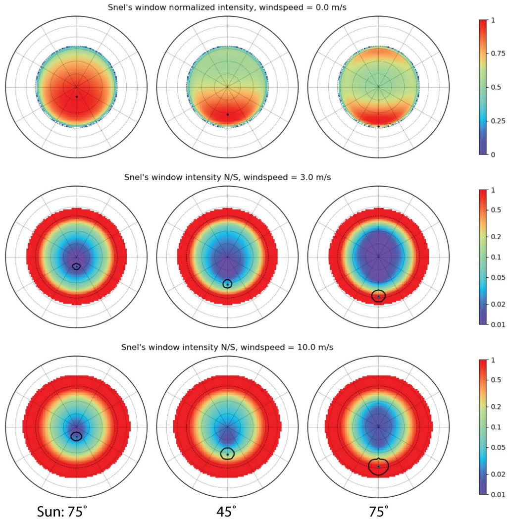
Figure 1. Simulated view of the sky through the water surface. Top row: normalized intensity, in false color. The sun's position is marked by a black dot. Middle and bottom rows: intensity noise due to waves at 3 m/s and 10 m/s wind speeds, respectively. The noise is normalized to the signal level to enable comparison. The contour around the sun's position surrounds the area that the sun's image is 99% likely to fall within. Each plot shows the entire hemisphere with the Lambert equal-area azimuthal projection—the centre is vertical and each concentric gridline is 15° down to the horizon. The extra dotted grid line is at 48°, the boundary of Snel's window with a flat surface.
