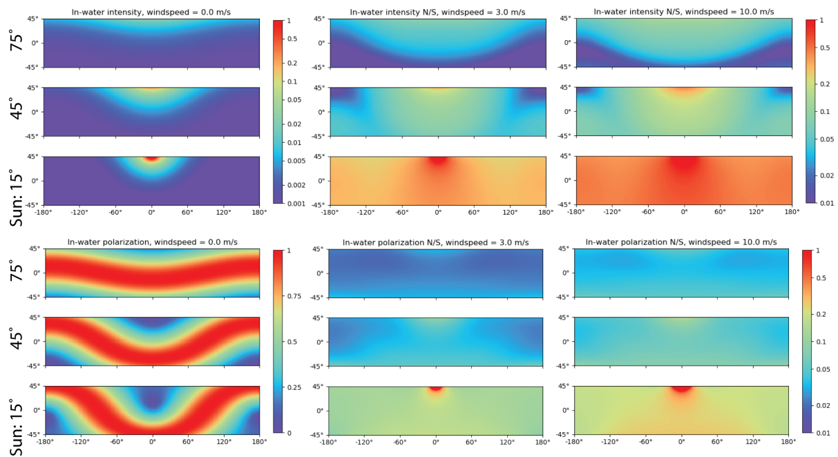
Figure 3. Scattered in-water light field. Left: patterns with a smooth water surface, middle: noise at 3 m/s wind, right: noise at 10 m/s wind. The noise levels are normalized to the signal so they can be compared. Top triplet: intensity, bottom triplet: polarization. The polarization variance is measured by treating the (S1, S2) vector as Rayleigh distributed.
