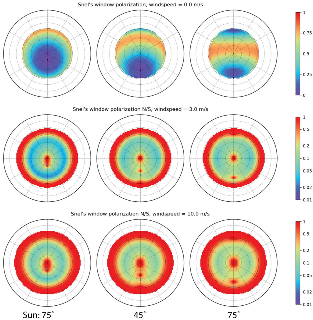
Figure 2. Simulated view of the sky through the water surface. Top row: degree of polarization. The sun's position is marked by a black dot. Middle and bottom rows: polarization noise due to waves at 3 m/s and 10 m/s wind speeds, respectively. The noise is normalized to the signal level to enable comparison. The polarization variance is measured by treating the (S1, S2) vector as Rayleigh distributed. Each plot shows the entire hemisphere with the Lambert equal-area azimuthal projection—the centre is vertical and each concentric gridline is 15° down to the horizon. The extra dotted grid line is at 48°, the boundary of Snel's window with a flat surface.
