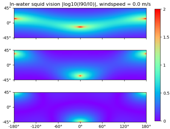
Figure 8. Squid's eye view of the scattered in-water light. Top to bottom: sun at 75°, 45°, and 15° elevation. The horizontal axis is the heading relative to the sun: the center is to the sun and the edges are away. Of note are the high-contrast spots at 0° and 180° heading, which would provide an easy navigation cue. Their elevation above and below the horizon is correlated to the elevation of the sun.
