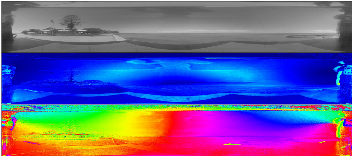
Figure 5. Catadioptric polarization imaging in air. Upper left: set-up with camera pointing down at a conical mirror with polarization filter tube, upper right: image captured by the set-up, lower strips: intensity image, degree of polarization, and polarization angle. In this case, the sun is blocked by the operator's body.
