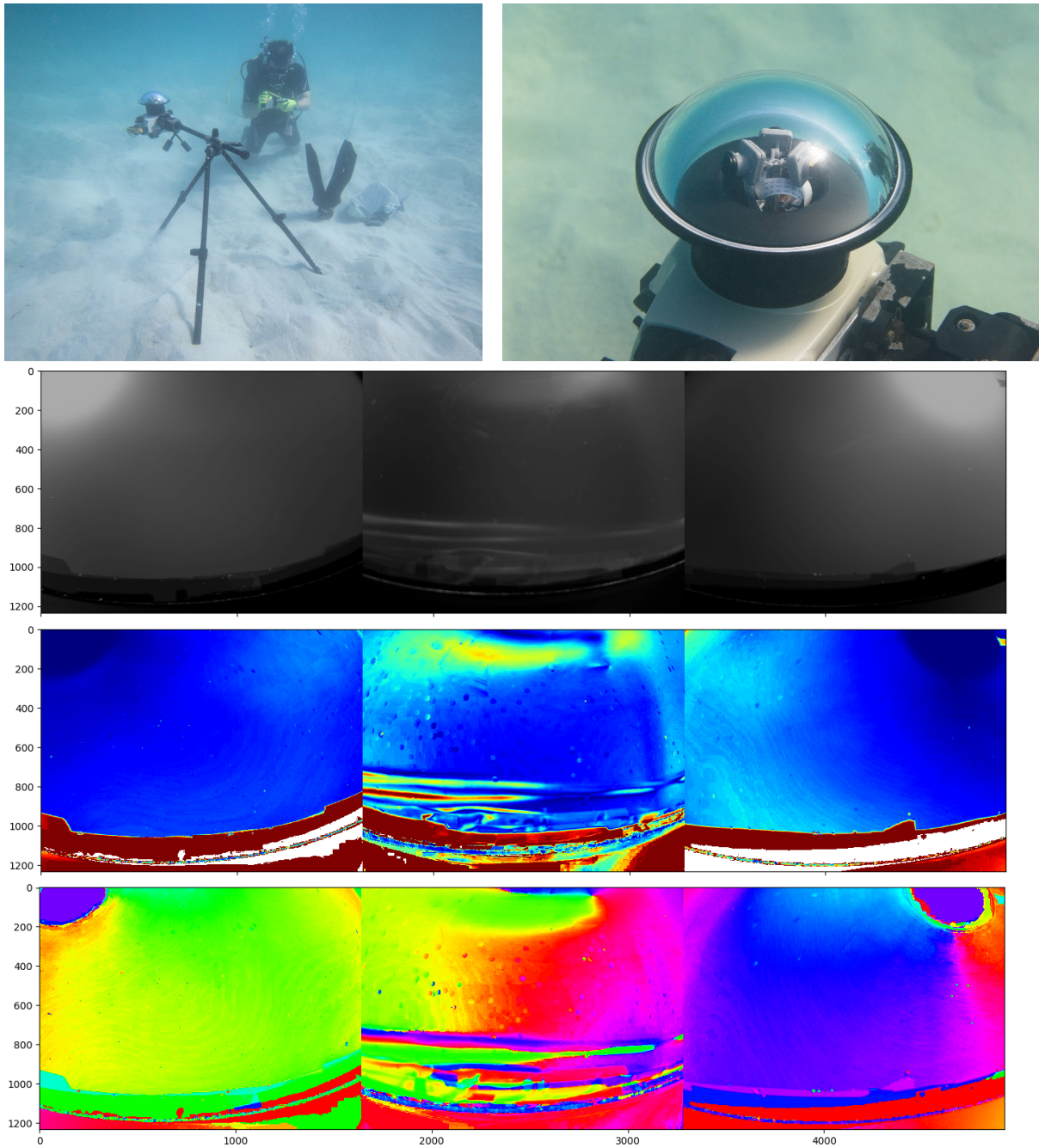
Figure 7. Multiple camera solution. Top: the camera system fits within a standard DSLR underwater housing. Bottom: intensity, degree of polarization and angle of polarization images. Bubbles and internal reflections from the polarizer tube (particularly visible in the center image) introduce confounding polarization signals, but the expected pattern is otherwise clearly visible.
