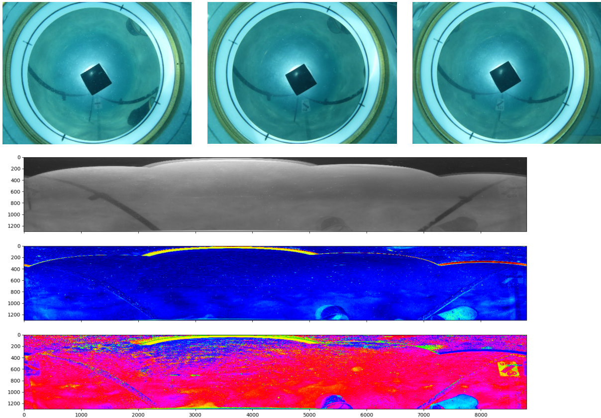
Figure 6. In the marine environment, the mirror tarnishes too quickly to obtain usable images, even when it's repolished before each dive. Top: images with each polarization filter (0°, 60°, 120°). A piece of vinyl tape blocks the reflection of the sun. Bottom: intensity, degree of polarization, and angle of polarization images—the noise from the tarnished mirror and slight shifts of the camera has destroyed any usable polarization signals.
