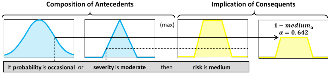
Figure 22. Example Implication of Consequents.
