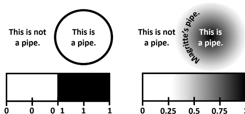
Figure 6. A Bivalent "Crisp" Set and a Multivalued "Fuzzy" Set.
