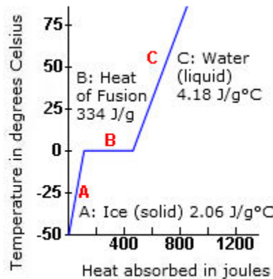
Figure 4.20 Energy Required for Ice Phase Change [40]
