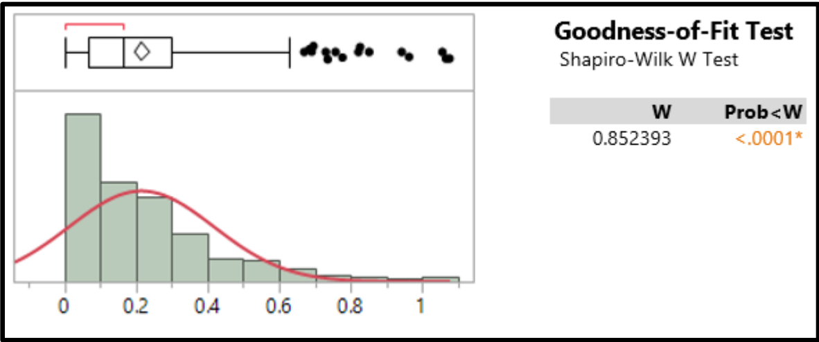
ST&E Shapiro-Wilk Test
