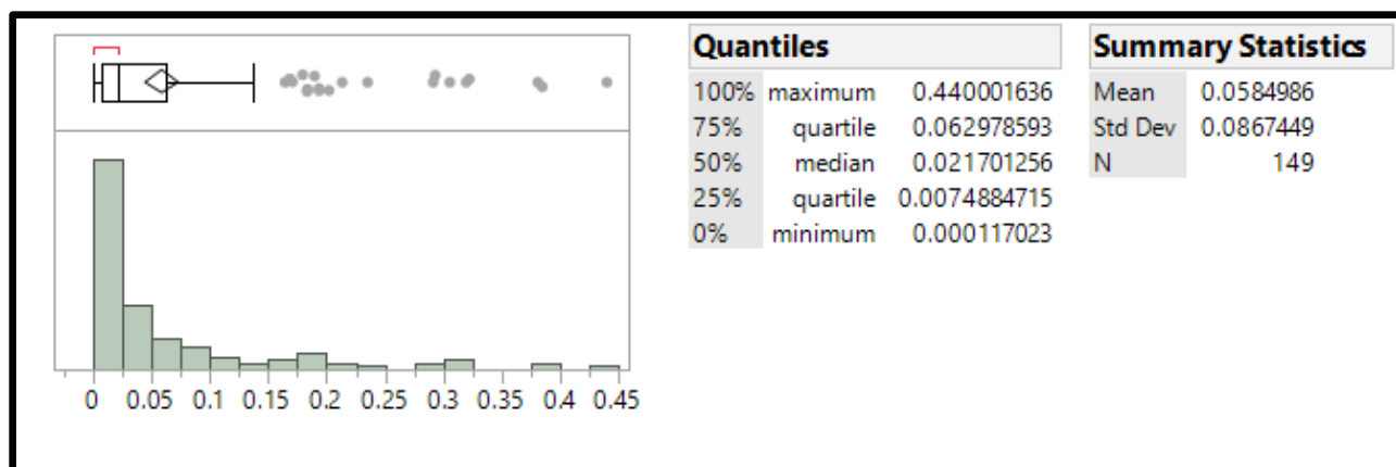
Figure 7. PSE Descriptive Statistics
