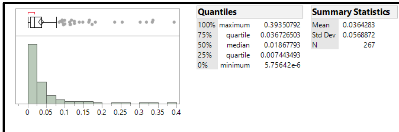
Figure 6. Data Descriptive Statistics
