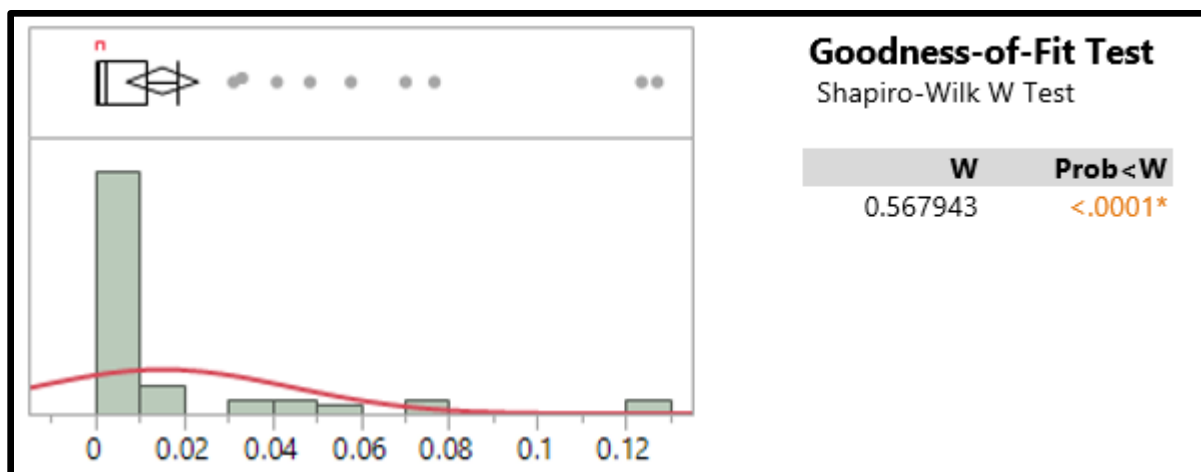
PSE Shapiro-Wilk Test
