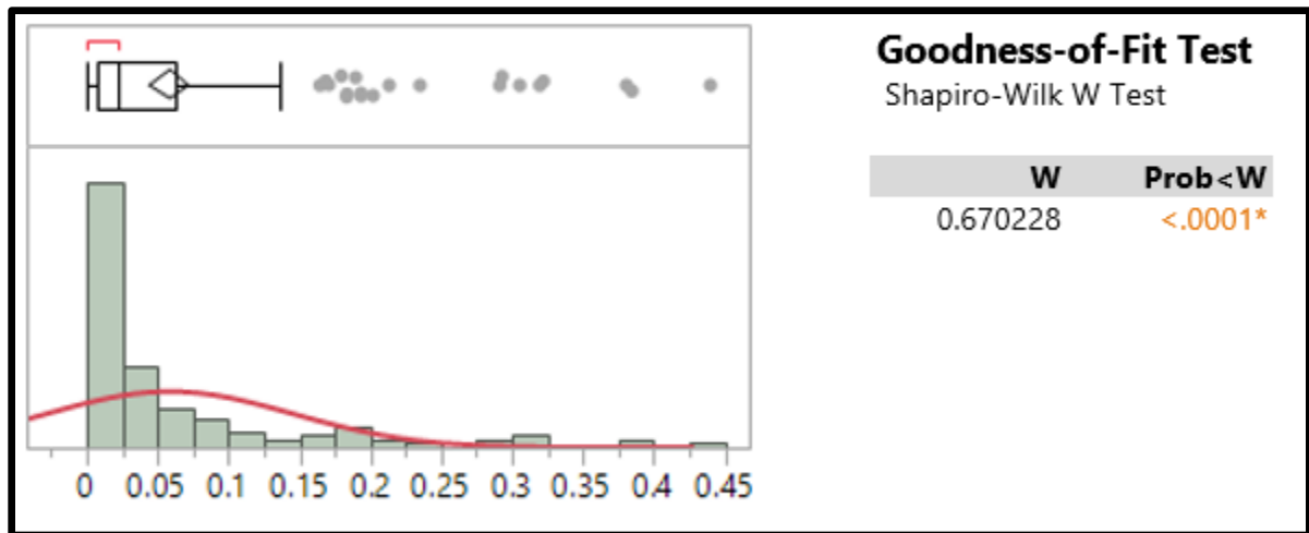
CSE Shapiro-Wilk Test
