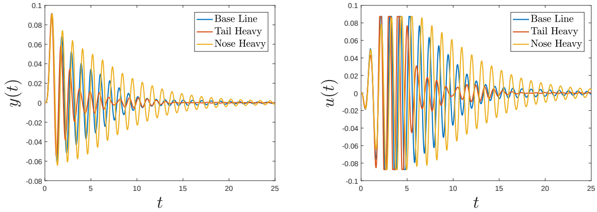
Figure 4.8: Closed-loop responses of aerofoils with the same design vector but varied centre of gravity and V_\infty = 4.5 \text{ m s}^{-1} . Centre of gravity is displaced a distance equal to 5% of the chord towards the tail in Tail Heavy case and displaced the same distance towards the nose for the Nose Heavy case.
