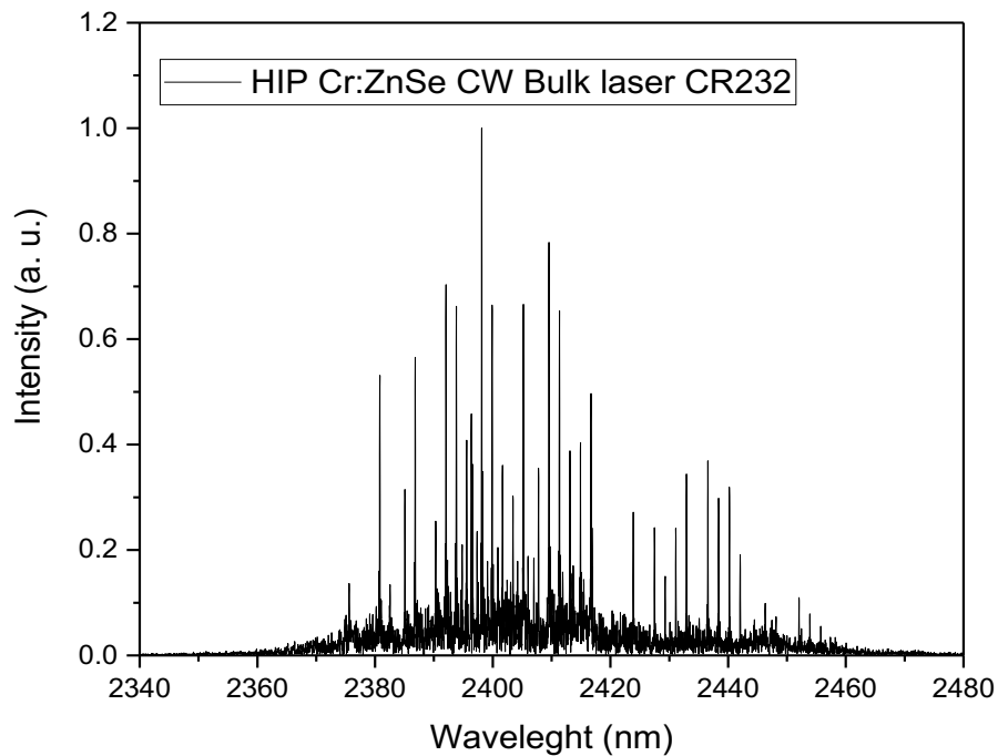
Figure 14. Spectral Emission from HIP CrZnSe bulk plane-plane cavity.
