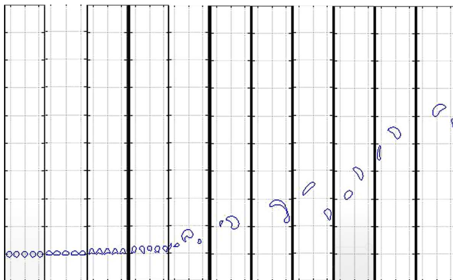
Figure 23: Simulation of an instantaneous puff behavior for a 5 bubbles flow inside the riser with volume correction.
