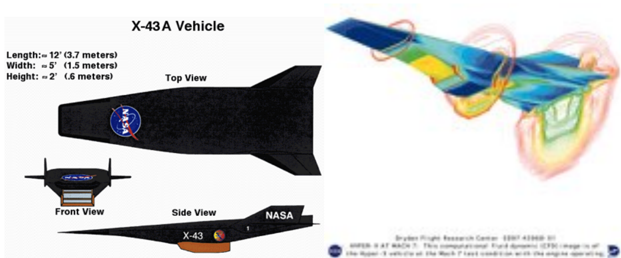
Figure 4. Figure 4. External expansion nozzle on the X-43 Hyper-X vehicle. (NASA).
