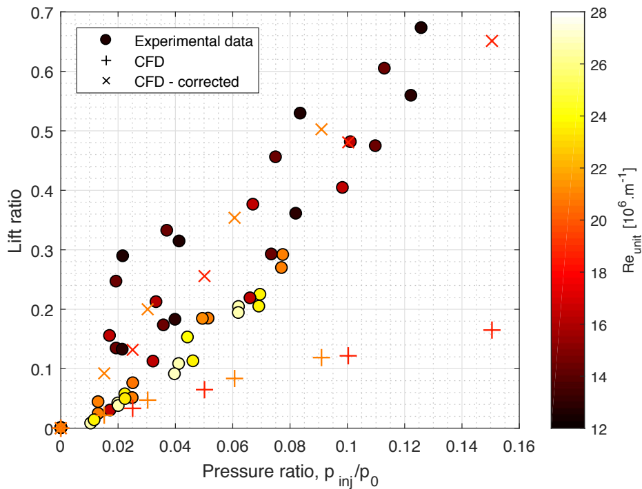
Figure 27. The dependence of lift ratio (eq. 2) on pressure ratio.
