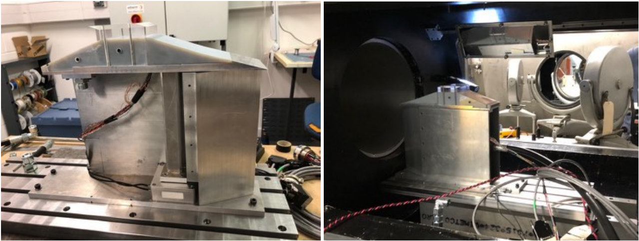
Figure 13. Photos showing the initial model configuration used in the Oxford HDT incorporating the long support arm joining the free floating model to the six-component load cell.
