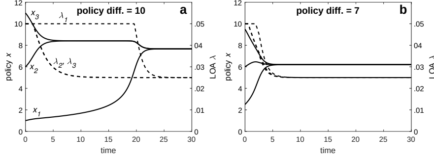
Fig. 3 Position and LOA trajectories in ASC model for a complete network. Solid curves show policy positions, dashed curves show LOAs. (a) High initial policy disagreement ( x_3 - x_1 = 10 ) showing substantial shift between consensus and initial mean policy ( x_2(0) ). (b) Lower initial policy disagreement (7) results in near simultaneous convergence close to initial policy mean. \lambda_{1,2,3}(0) = 0.05 , \lambda_{min} = 0.025 ; \rho(x) as in Fig. 2.
