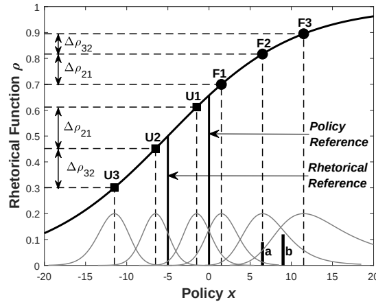
Fig. 2 Effect of rhetorical function concavity and offset reference. \rho(x) = 1/(1 + e^{-\beta(x-x_0)}) with \beta = 0.13 , x_0 = -5 . Short lines at bottom show alternative F group consensus policies: (a) mean policy \bar{x} = x_2 ; (b) RPM policy \bar{x}_{23} = (x_2 + x_3)/2 . ASC model acceptance functions in gray.
