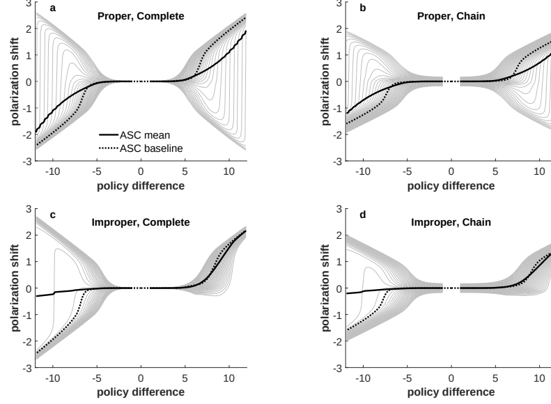
Fig. 4 ASC simulations for triad networks with variability in intermediate node policy. \rho(x) taken as in Fig. 2. Top row shows proper rhetorical frame ( x_0 = 0 ). Bottom row shows improper rhetorical frame ( x_0 = -5 ). Positive and negative policy sides are on positive and negative horizontal axis respectively. Polarization shift, \delta = \bar{x}(t_f) - \bar{x}(0) , plotted as a function of the initial policy difference, \Delta = x_3(0) - x_1(0) . Shift toward the extreme corresponds to \delta > 0 for positive policy side and \delta < 0 for negative side. The position of the intermediate node was varied according to x_2(0) = \pm(6 + \epsilon) for the positive and negative policy sides, where \epsilon takes on 41 uniformly-spaced values over the interval [-1, 1] . x_1(0) = 6 - \Delta/2 and x_3(0) = 6 + \Delta/2 for \Delta > 0 and analogously for \Delta < 0 . ASC mean (black) taken over all \epsilon values. Shifts for individual \epsilon values shown as gray curves. Dotted curve shows \epsilon = 0 baseline case where x_2(0) = 6 . Gap in the curves is the region where x_2(0) would go beyond x_1(0) or x_3(0) . ASC model parameters: \lambda_{1,2,3}(0) = 0.05 , \lambda_{min} = 0.025 .
