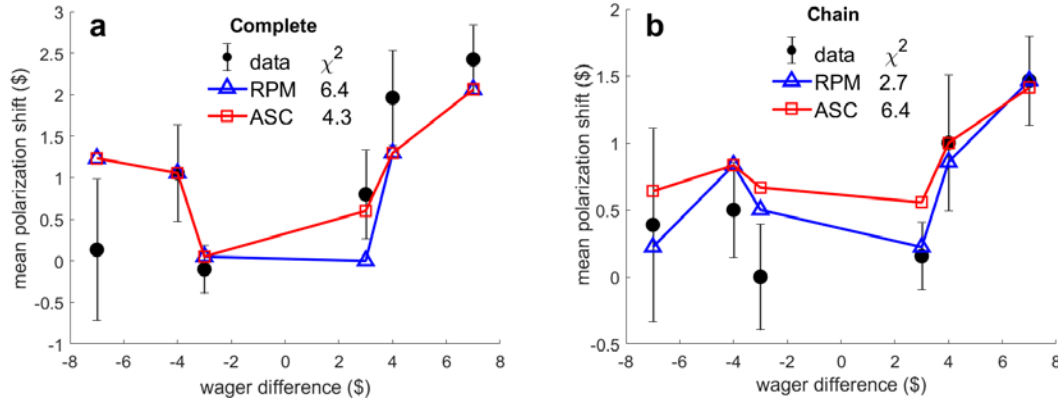
Figure 4. Comparison of experimental data and simulations of ASC and RPM models. (a) Complete network. (b) Chain. Positive and negative sides of the x-axis correspond to favorite and underdog groups respectively. Error bars are standard errors. Simulation results are rounded upward to nearest dollar.
