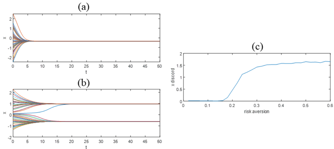
Figure 3. ASC model simulations for large network showing transition between convergent and divergent behavior. Opinion vs. time for (a) low risk aversion of 0.1 and (b) high risk aversion of 0.35. (c) Final policy discord vs. risk aversion showing transition between convergence and divergence at risk aversion of 0.16. A complete network topology of 51 nodes was used.
