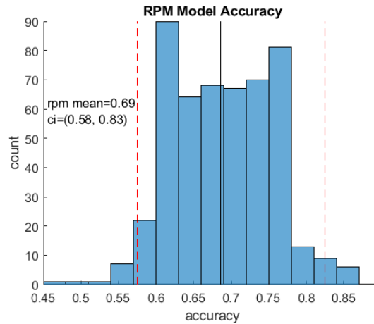
Figure 5. Distribution of RPM model accuracy in predicting polarization out of sample over 500 samples. Training set size = 40 groups. Test set = 119 groups.
