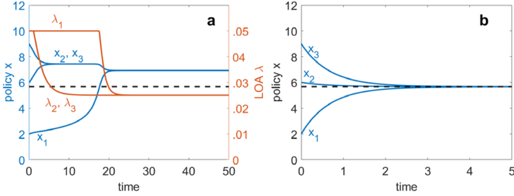
Figure 2. Evolution of policy positions and uncertainties for completely-connected triad. (a) ASC model. (b) Consensus protocol. Dashed lines indicate initial mean policy.
