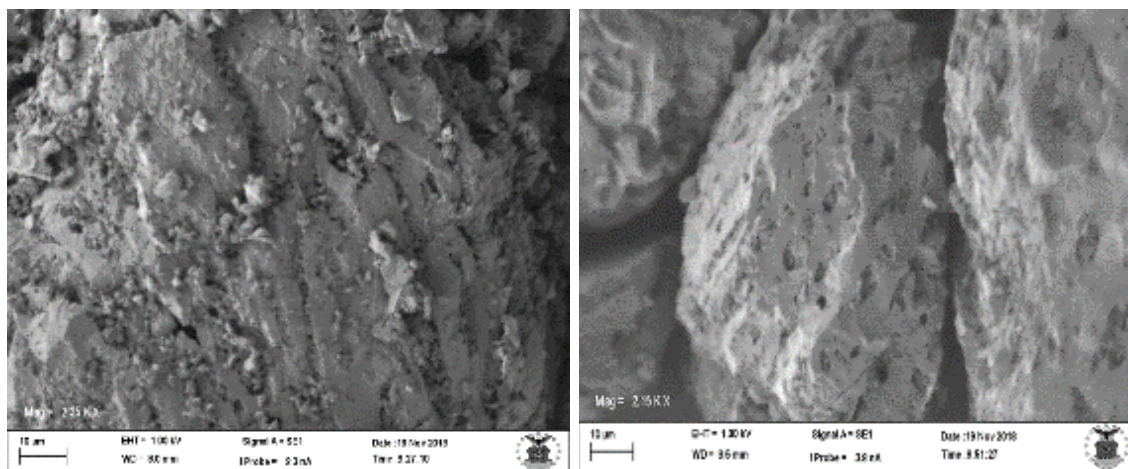
Figure 20. Evoqua AquaCarb® 1230CX as is (on the left) and modified (on the right) SEM images showing the external surfaces and overall structure of the GAC magnified at 2.35 KX (on the left) and 2.15 KX (on the right) respectively.
