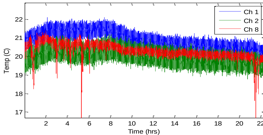
Figure 16: Thermal measurements from the day identification measurements were done.
