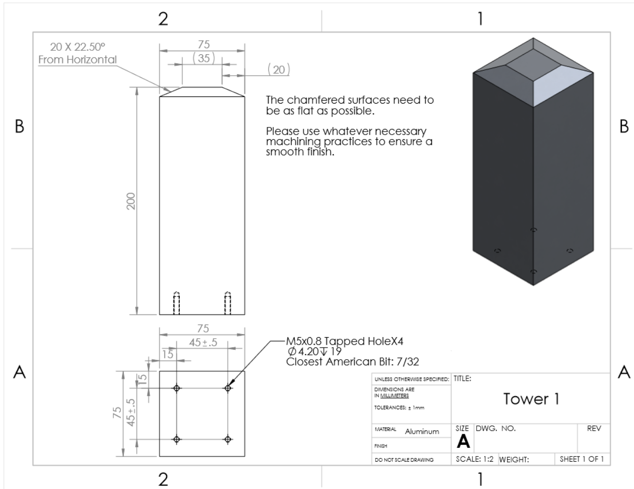
Figure 55: Calibration Piece
