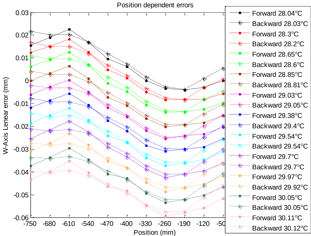
Figure 11: Linear errors along W axis with respect to positions from B5 test.
