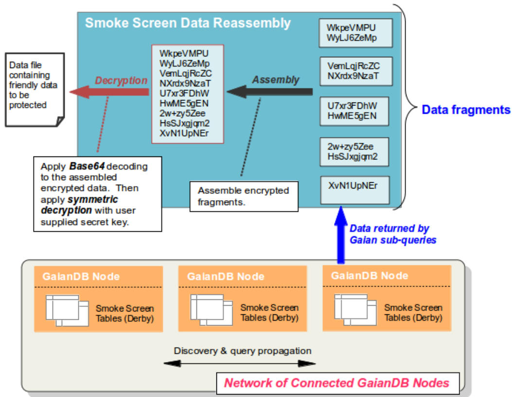
Fig. 5 Smoke Screen data reassembly processing
