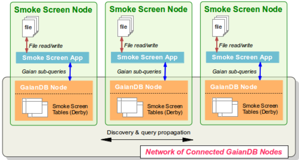
Fig. 1 Smoke Screen architecture
