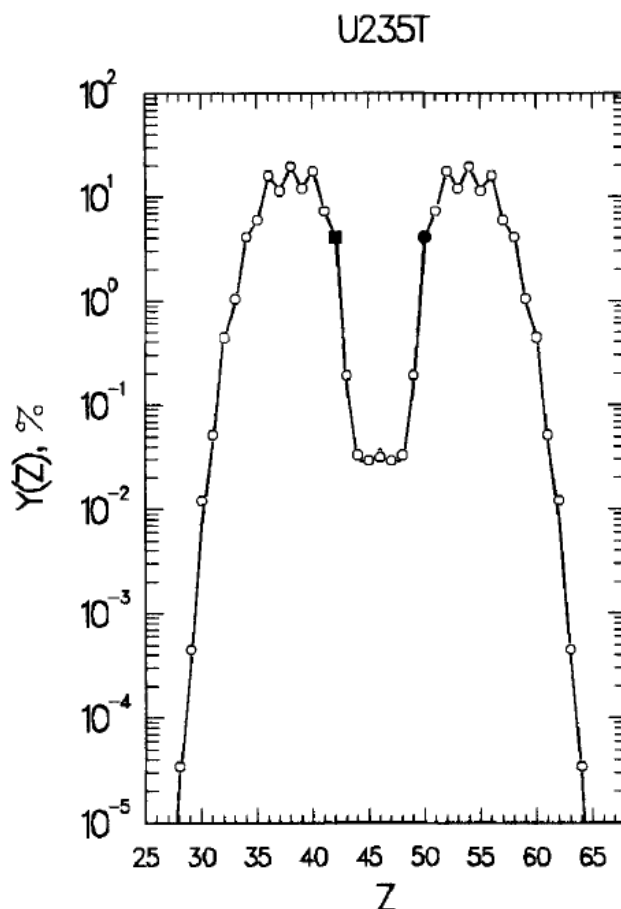
Figure 1. The characteristic double-hump curve of the fission of uranium-235 into its potential fission fragments. The process is statistical in nature, and the probability of the resulting products is given on the vertical axis. This is reproduced from Wahl (1988).
