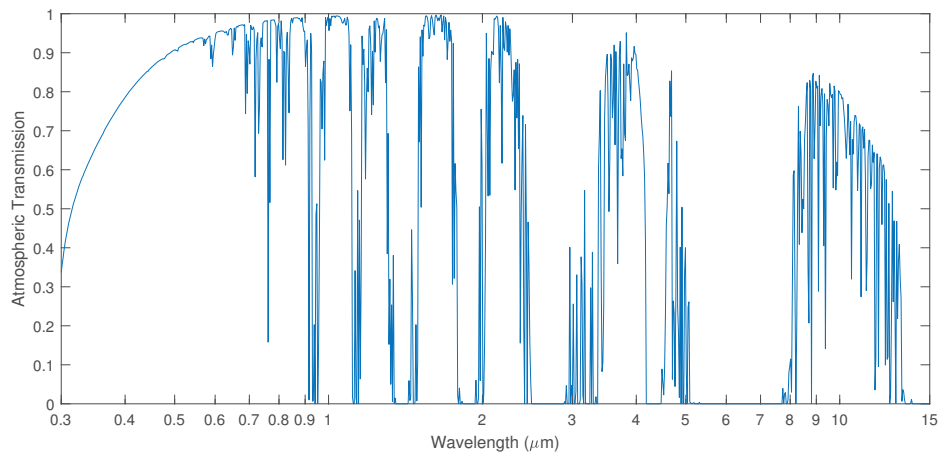
Figure 8. The figure shows how transmission of light is affected by the various constituents present in the atmosphere.
