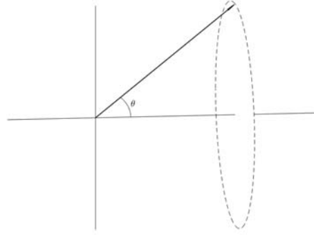
(b) Scattering is dependent only on the angle \theta and can occur at any azimuthal angle on the dashed circle
