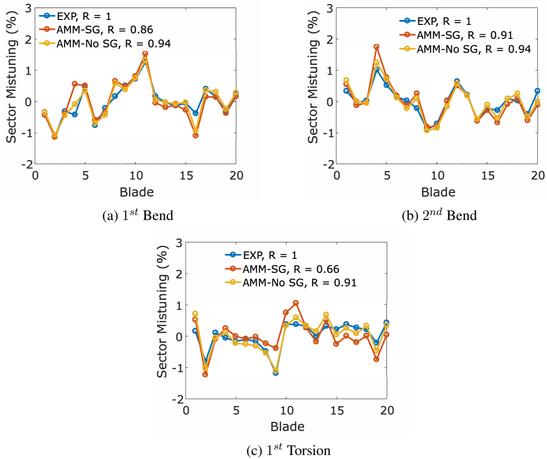
Figure 6.8: Modal Ping Testing Sector Mistuning
