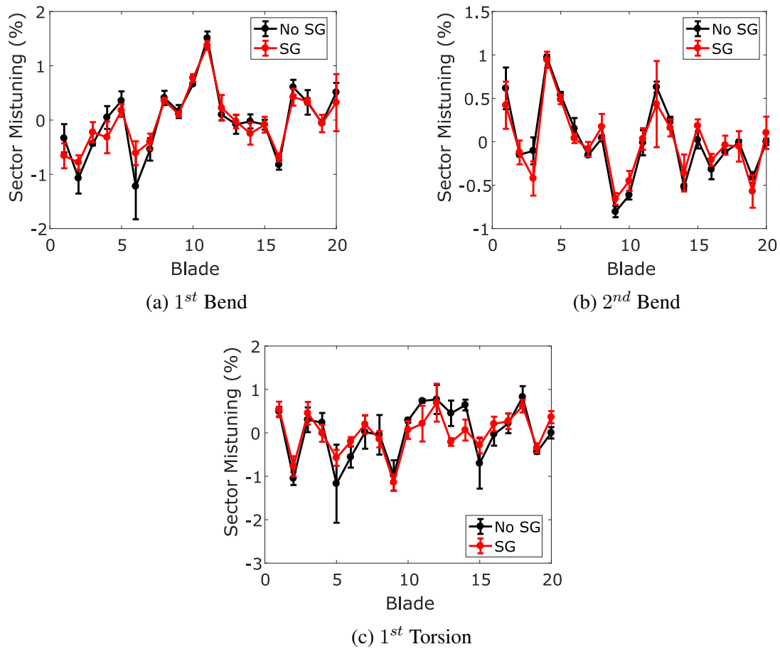
Figure 6.14: PBS R4 EO9 Sector Mistuning
