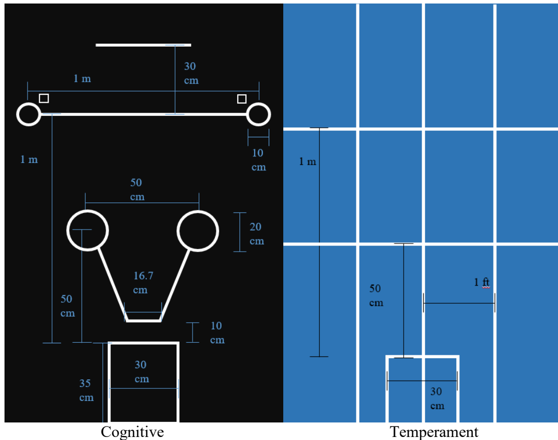
Figure 9. Mat Diagrams
