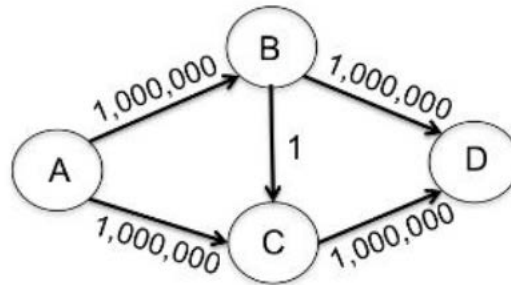
Figure 3: Standard example graph that allegedly exhibits the worst-case performance of the Ford-Fulkerson method.
