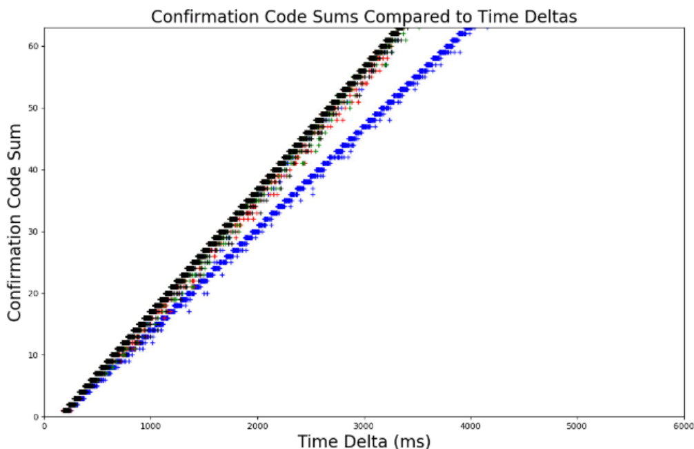
Figure 9: InAndOut timing side channel inconsistencies: confirmation number vs response delay (milis). The graph consists of 11988 orders. The first 3000 orders placed are shown in blue.
