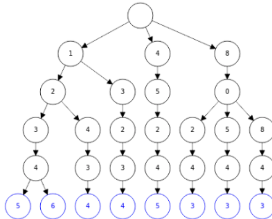
Figure 6: Example of a trie containing numbers: 12346, 12345, 12434, 13234, 45245, 80243, 80543, and 80843.
