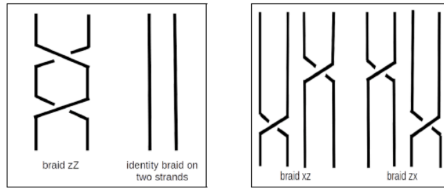
(a) Consecutive inverse operations are equivalent to the identity braid: zZ = \varepsilon .
