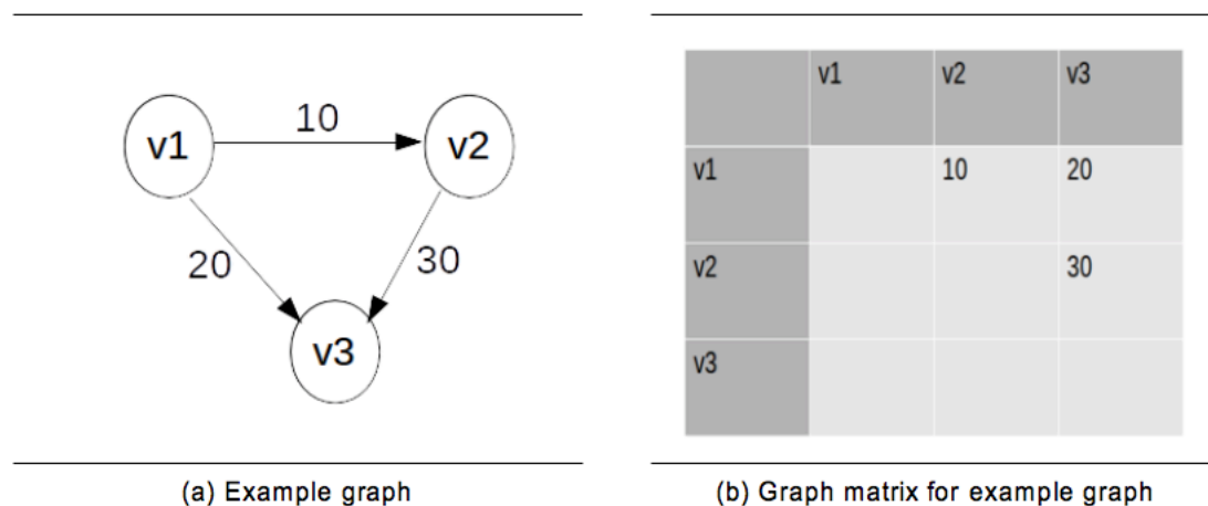
Figure 4: A graph and its matrix representation.
