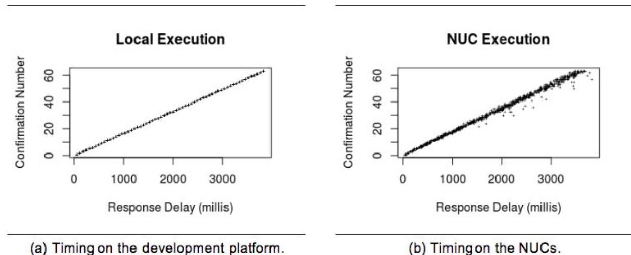
Figure 10: The Confirmation Number Timing Side Channel in InAndOut.
