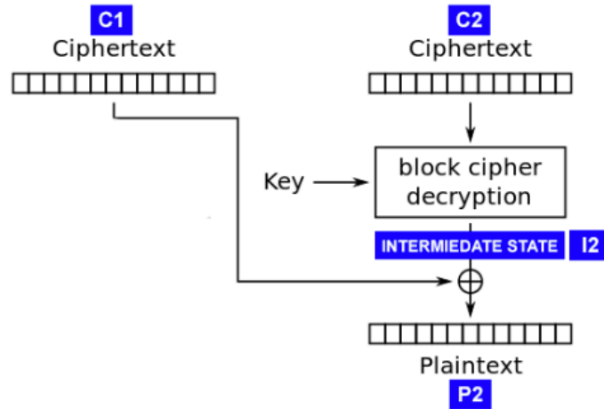
Figure 8: The intermediate state in CBC mode decryption.
