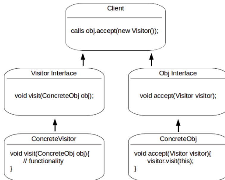
Figure 2: Diagram of the Visitor Pattern in Java
