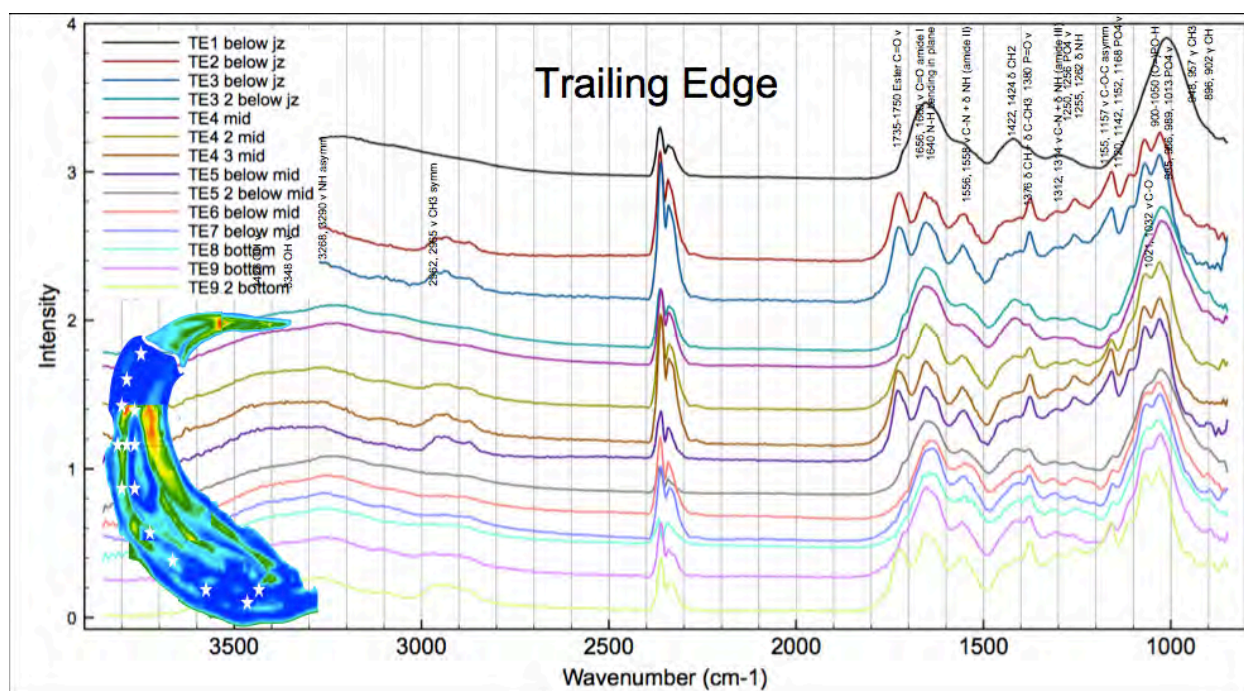
Figure 35. FTIR mapping of trailing edge of tooth along length of stylus.
