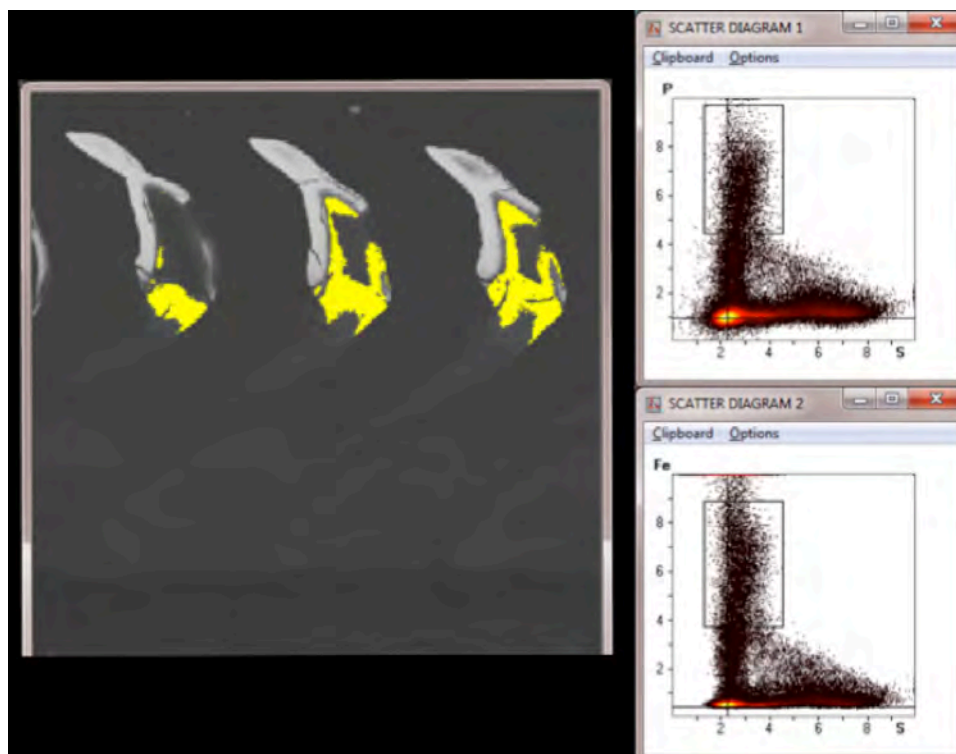
Figure 26. Energy Dispersive Spectroscopy map (left) from highlighted Fe and P-rich nodes (right) in less mineralized teeth from the S3 region.
