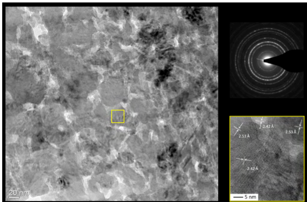
Figure 19. TEM analysis of outermost particle region of leading edge of tooth.
