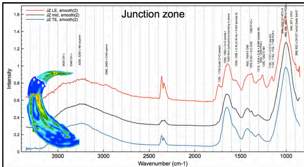
Figure 33. FTIR mapping of junction zone of tooth along leading, middle and trailing edges.
