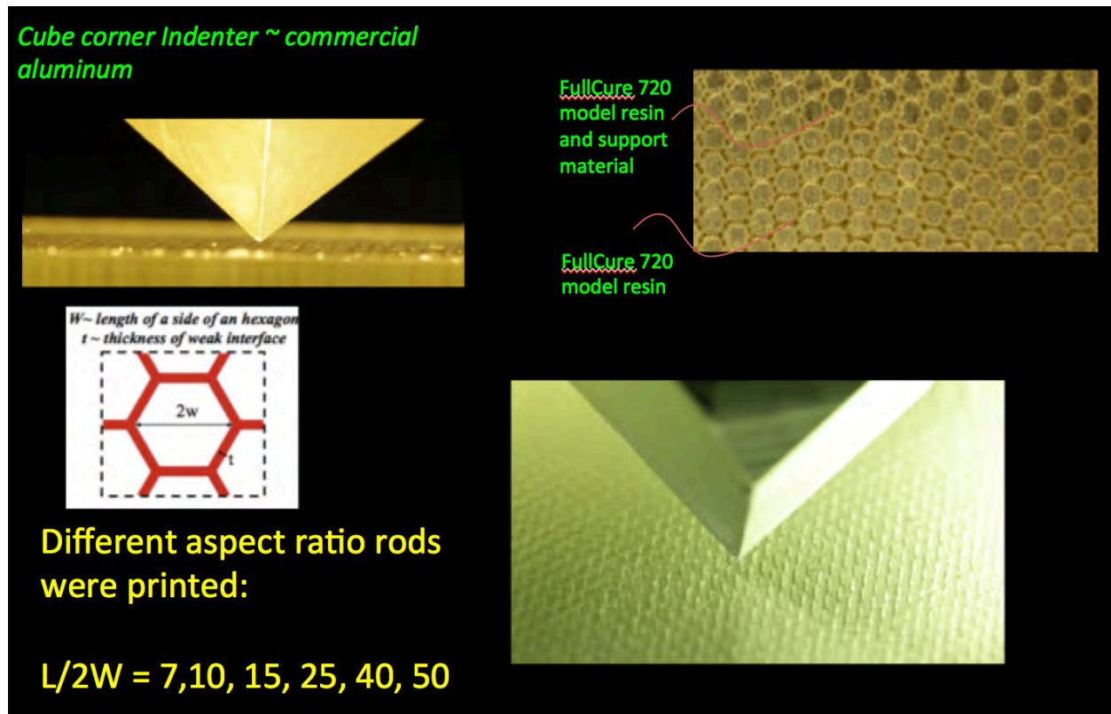
Figure 23. 3D printed mimics of shell region of chiton teeth. Samples were made with different rod aspect ratios (Length / 2 x width): 7, 10, 15, 25, 40, 50 and indented to determine optimized aspect ratio for abrasion resistance.
