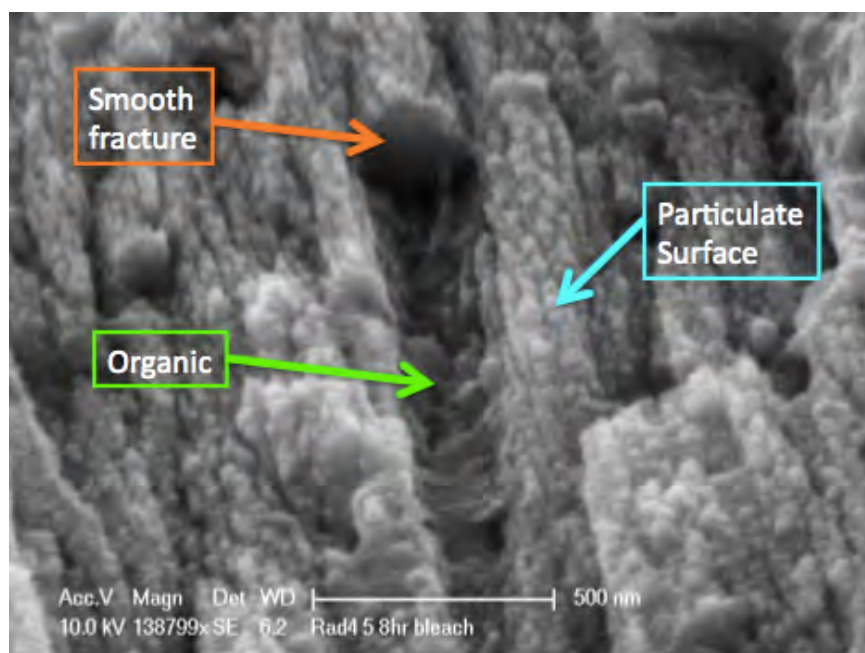
Figure 21. SEM observations of fractured region in shell with nanorod pullout that highlights
