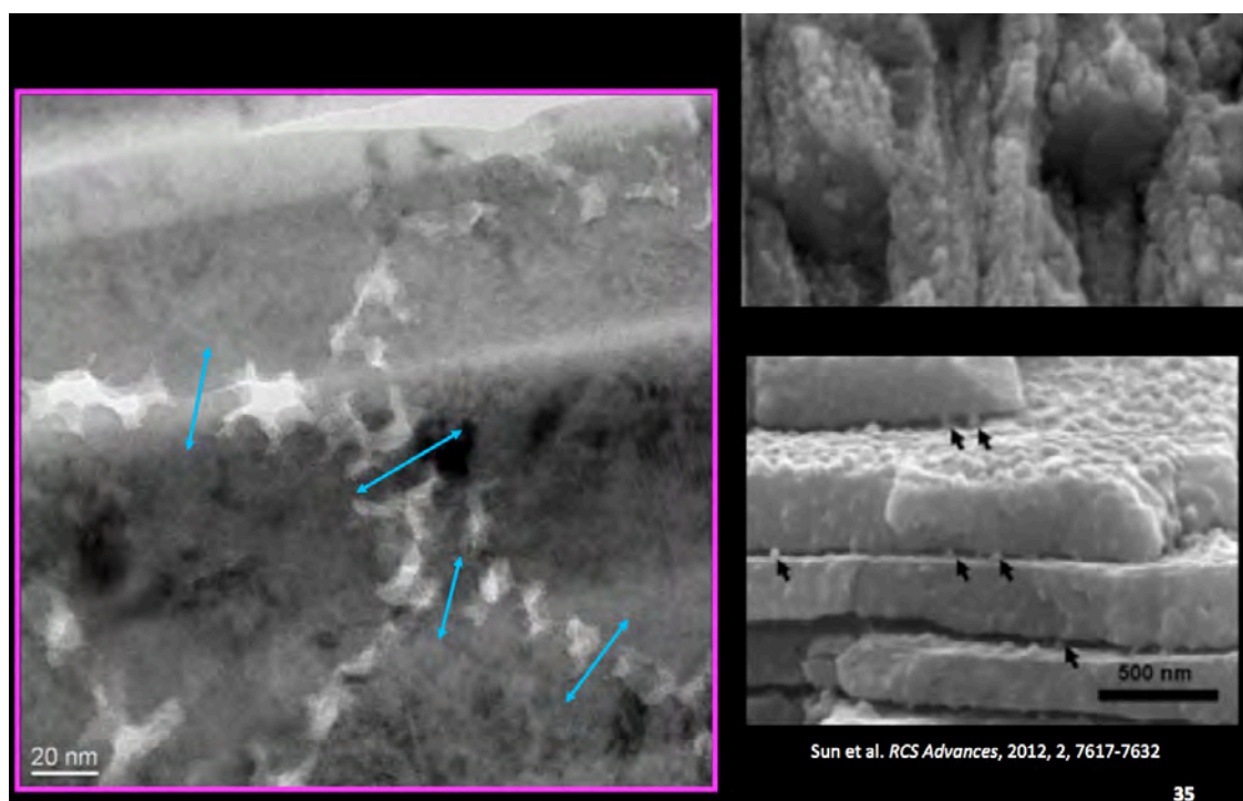
Figure 21. TEM analysis of the nanorod region from the leading edge, highlighting the presence of mineral bridges (left). SEM of the surface of the rods (upper, right) highlighting nanoasperities, which are similar to those seen in nacre tablets (lower, right).
