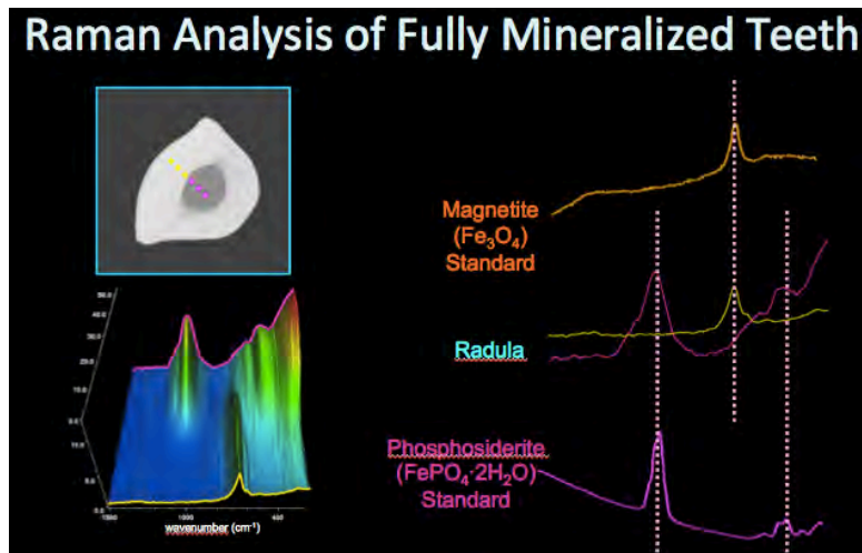
Figure 7. Line scan analysis of the core and shell regions of the fully mineralized teeth with Raman spectroscopy.
