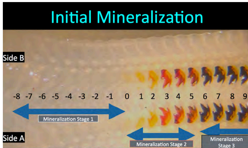
Figure 10. Initial section of the radula from the Chiton, showing the transition from non-mineralized teeth that consist of an organic framework (Stage 1) to the initial stage of mineralization (Stage 2) where Teeth are capped by a reddish brown hydrous oxide material, ferrihydrite ( 5\text{Fe}_2\text{O}_3 \cdot 9\text{H}_2\text{O} ) and the Transformation to magnetite is initiated in Stage 3.
