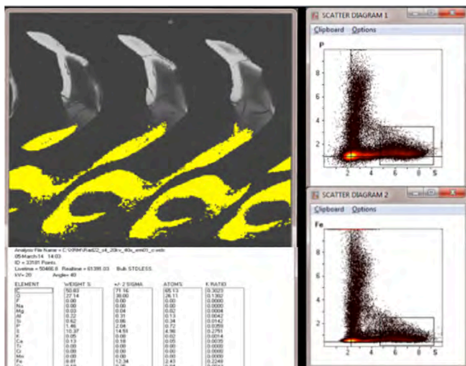
Figure 25. Energy Dispersive Spectroscopy map (left) from highlighted sulfur rich nodes (right).
