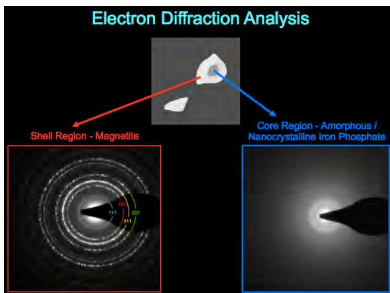
Figure 8. Electron diffraction analyses of shell (left) and core (right) regions.
