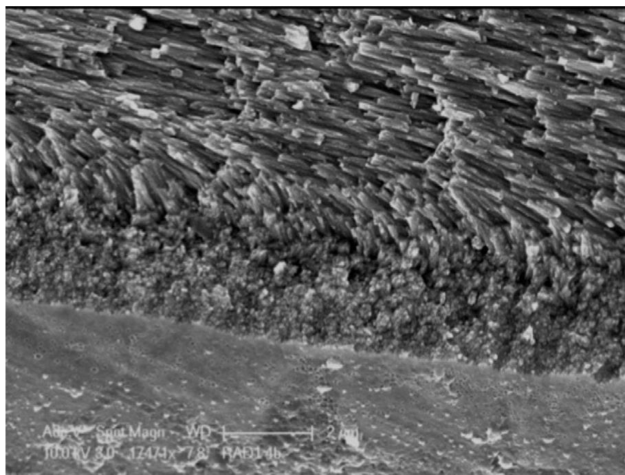
Figure 15. SEM analysis of the leading edge of a fully mineralized tooth. The outermost layer consists of randomly oriented particles where randomly organic existed whereas oriented rods exist within the surface.
