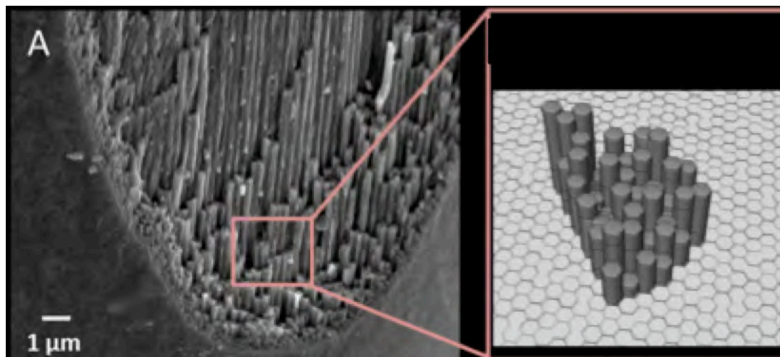
Figure 22. Rod like structure from shell region of teeth and finite element model.
