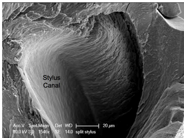
Figure 31. SEM micrograph of fractured stylus highlighting canal region.
