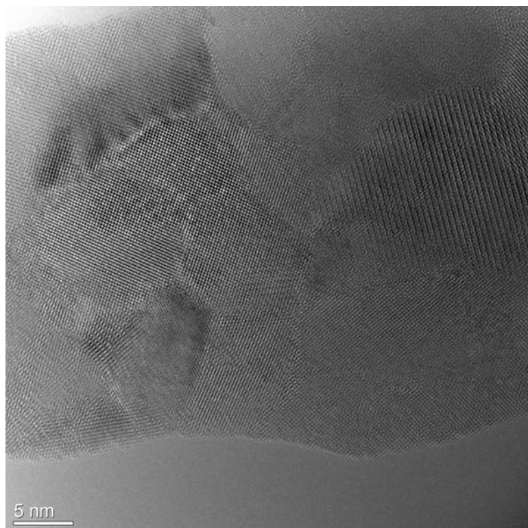
Figure 6. High resolution TEM of mineral from shell region, highlighting presence of nanograins of mineral.
