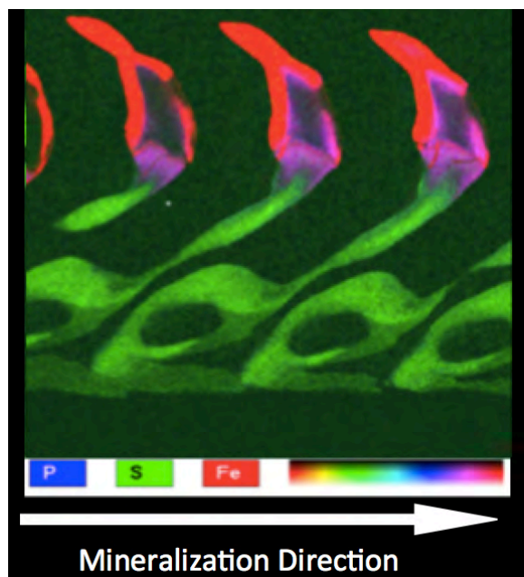
Figure 23. Energy Dispersive Spectroscopy of chiton teeth highlighting the increase in Fe and P species into the core of the tooth from the stylus.
