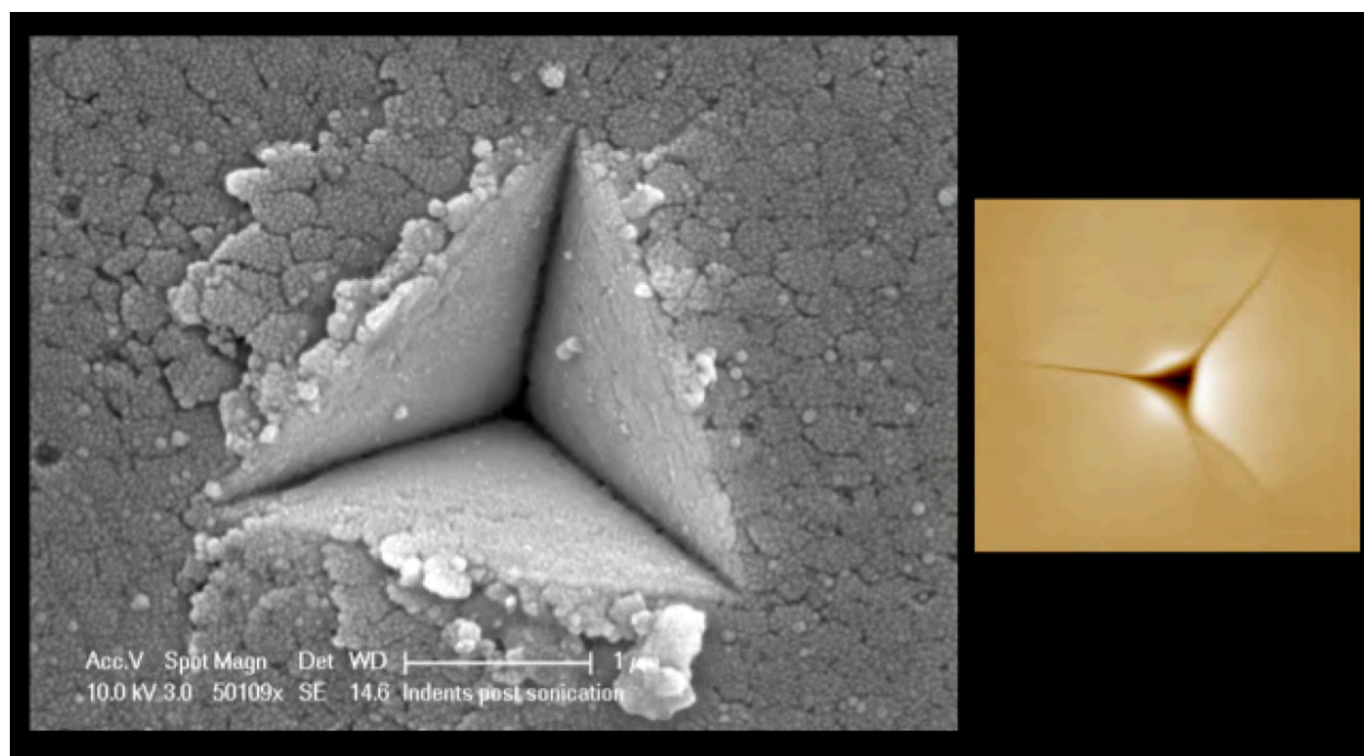
Figure 20. SEM observations of transverse section of the tooth at an indentation, revealing cracks that propagate around nanorods. The sample shown here was indented using a sharp cube-corner tip to induce cracking. After indentation, the sample was sonicated in acetone. Cracks can be seen to propagate between mineralized rods, rather than radially outward as is common with this type of indentation (shown on glass on the right).
