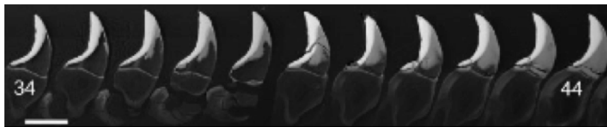
Figure 22. Back Scattered SEM of chiton teeth from row #34 - #44. Clearly the core is becoming mineralized.
