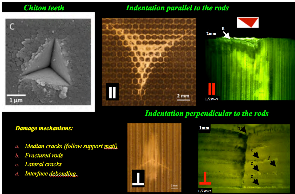
Figure 24. Results of indentation tests of biomimetic chiton teeth shells.
