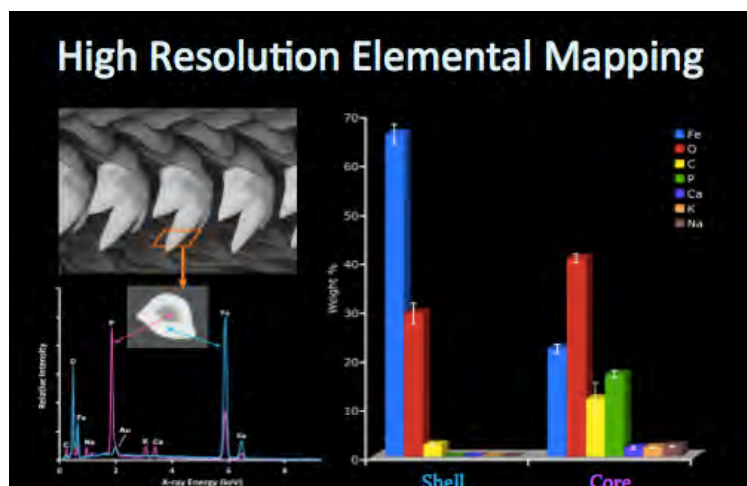
Figure 4. High-resolution EDS analysis of core and shell regions.
