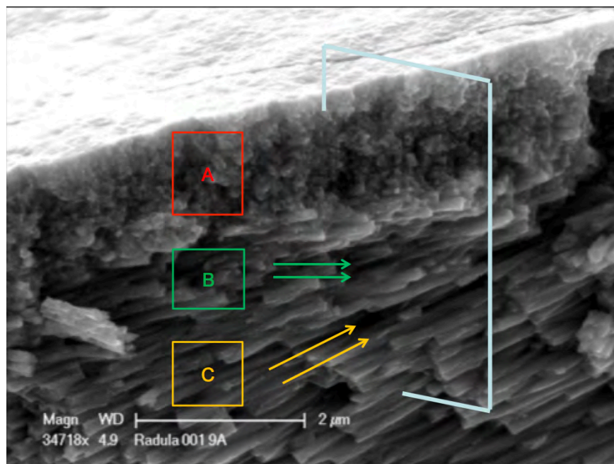
Figure 18. Region of leading edge of tooth selected for FIB sectioning in order to analyze using TEM.
