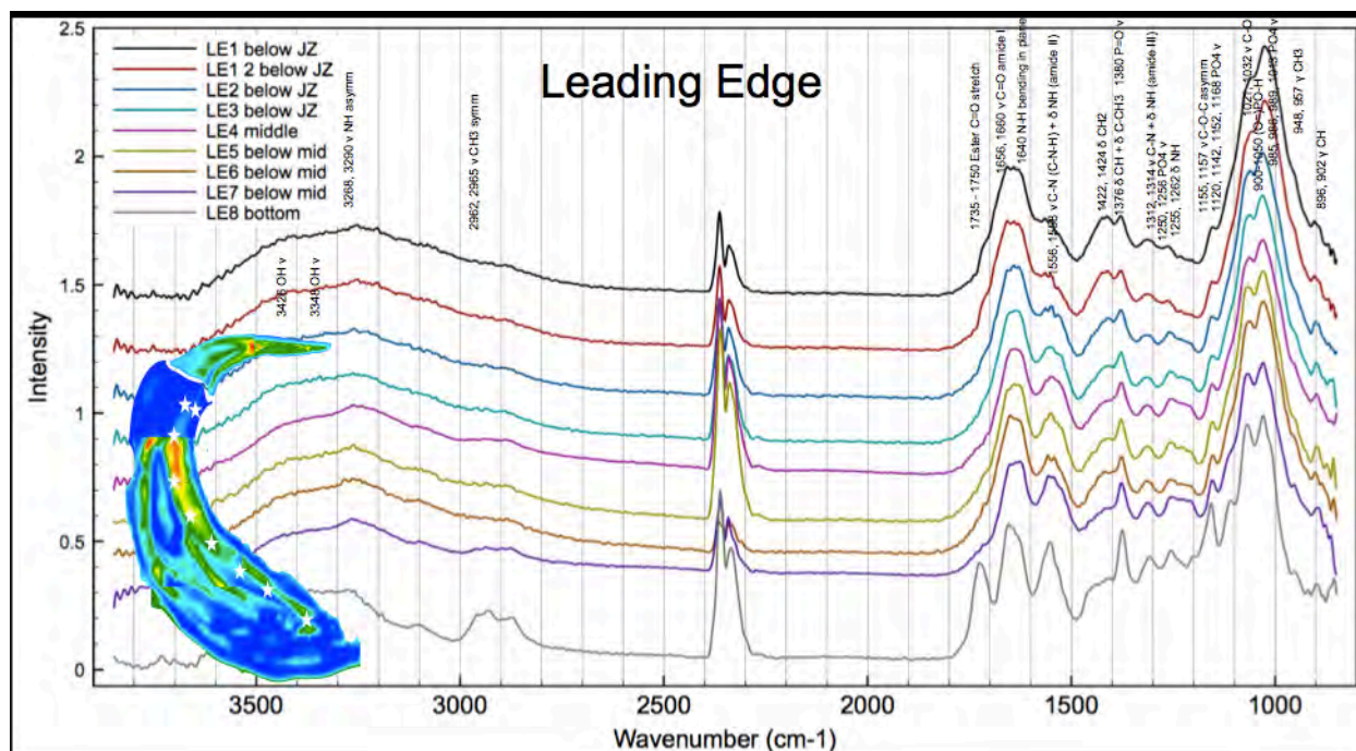
Figure 34. FTIR mapping of leading edge of tooth along length of stylus.
