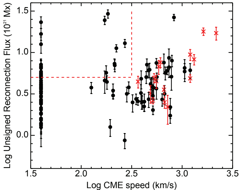
Figure 4. Log-log lots of the flare unsigned reconnection fluxes versus the CME speeds for the 126 flares. Black dots are flares with no associated SEP events, and red crosses are the 15 flares with SEP events. The flares with log CME speed = 1.6 are cases of no associated CMEs, for which V_{cme} was taken as 40 km/sec. The best candidates for flare SEP events are those in the upper left quadrant indicated by dashed lines. Plot units of the reconnection fluxes and CME speeds are 10^{21} Maxwells and km/sec, respectively.
